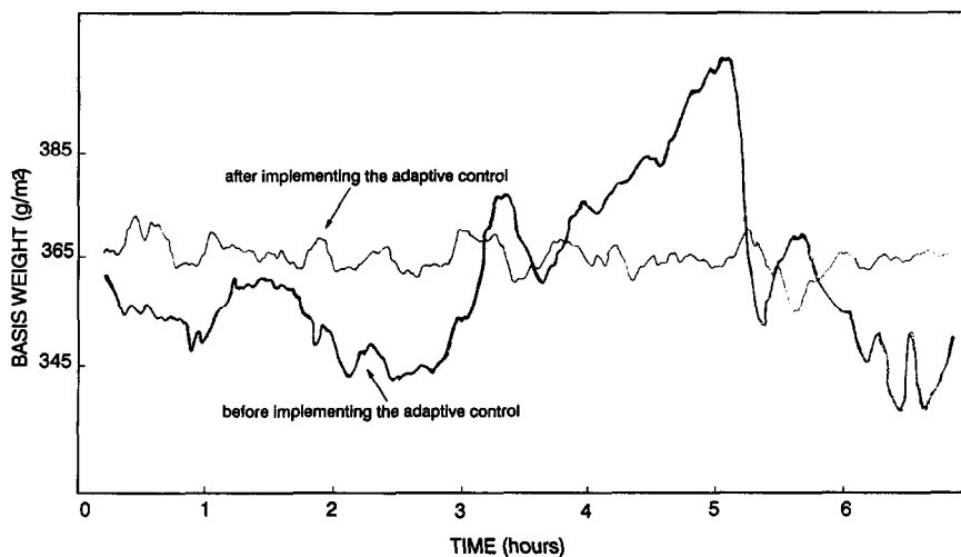
Figure 5 Comparison of basis weight variation before and after implementing the adaptive control
