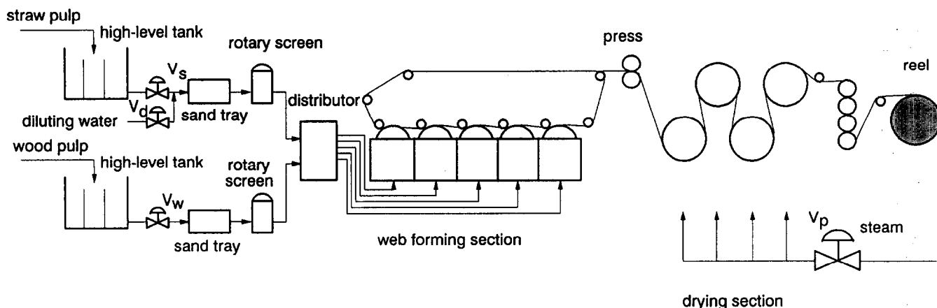
Figure 1 Flow diagram of the paperboard machine
