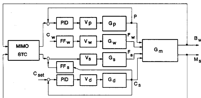
Figure 2 Adaptive control strategy for the paperboard machine
