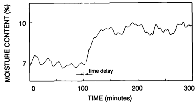
Figure 4 Response of moisture content when setpoint changes
