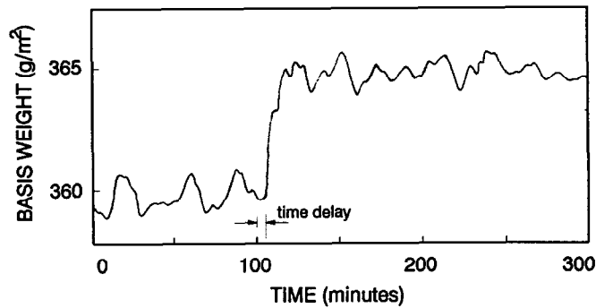
Figure 3 Response of basis weight when setpoint changes
