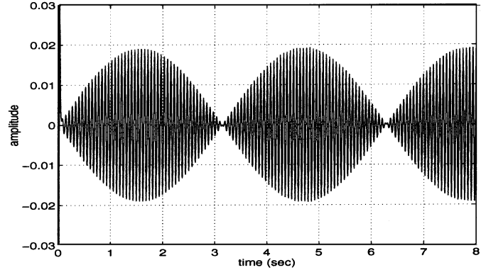
Fig. 11. Decrypted message f(t) = 0.02 \sin(t) \sin(100t) .
