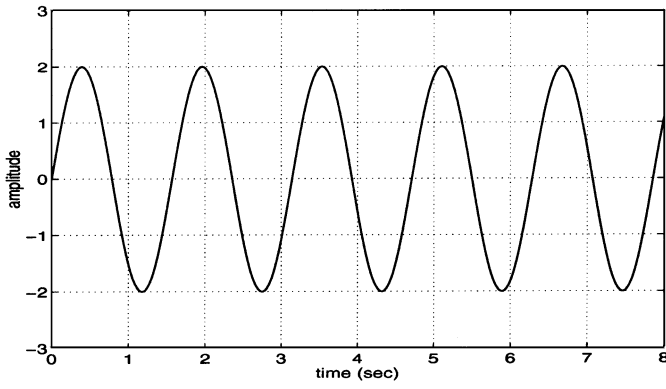
Fig. 8. Original message f(t) = 2 \sin(4t) before encryption.
