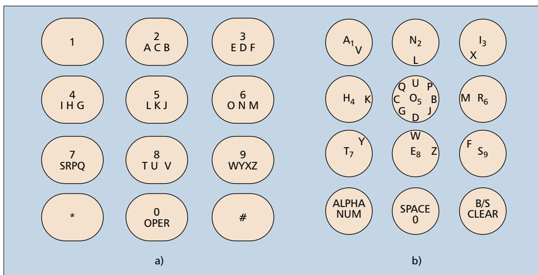
■ Figure 2. Keypad layouts: a) Less-Tap ; b) MessagEase .
