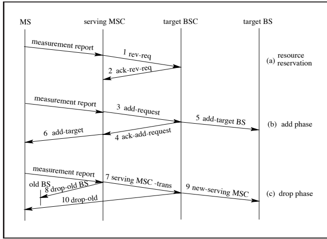
Figure 2: Soft handoff signalling.
