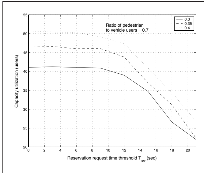
Figure 10: Capacity utilization vs. reservation-request time thresholds with the new call arrival rate being 0.3, 0.35 and 0.4.
