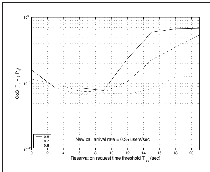
Figure 7: GoS performance vs. reservation-request time thresholds with the ratio of pedestrian to vehicle users being 0.8, 0.7 and 0.6.
