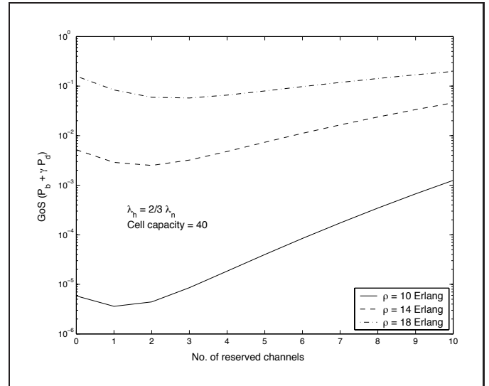
Figure 4: GoS vs. number of reserved channels.
