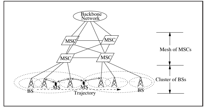
Figure 1: Network structure.
