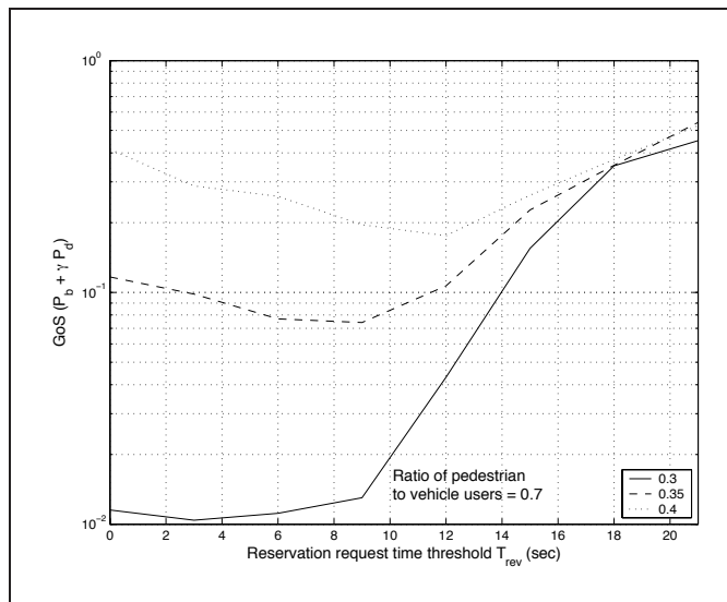
Figure 9: GoS performance vs. reservation-request time thresholds with the new call arrival rate being 0.3, 0.35 and 0.4.
