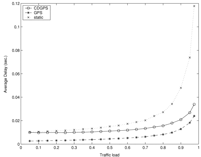
Fig. 4. Average delay comparison.
