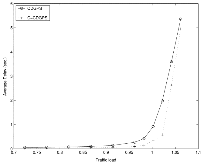
Fig. 8. Average delay comparison: CDGPS and C-CDGPS.
