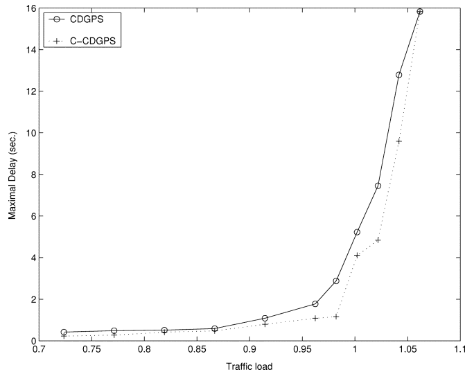
Fig. 9. Maximum delay comparison: CDGPS and C-CDGPS.
