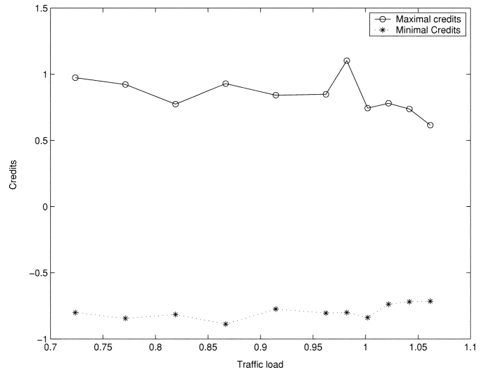
Fig. 10. Maximum and minimum credits in C-CDGPS.
