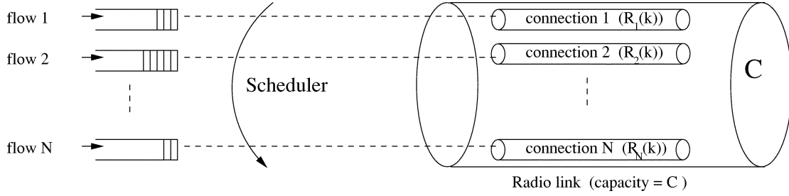
Fig. 3. Queueing model of CDGPS scheme.
