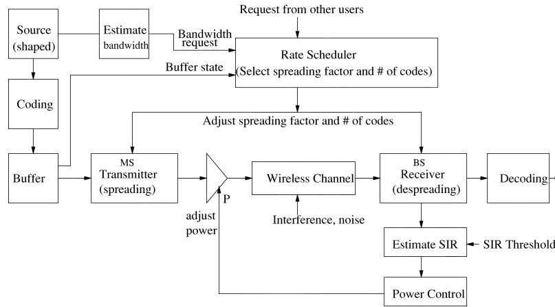
Fig. 1. Rate-scheduled wideband DS-CDMA system.
