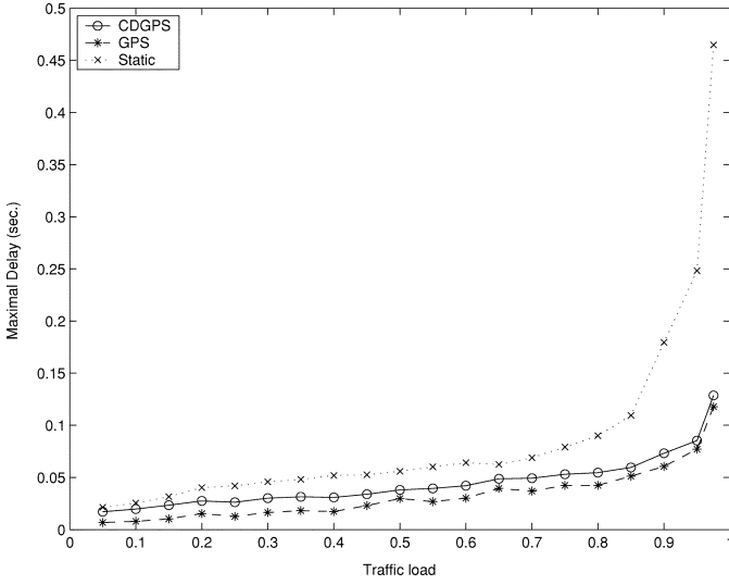
Fig. 5. Maximum delay comparison.
