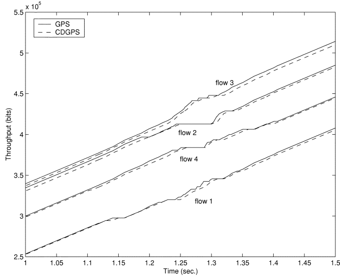
Fig. 6. Throughput comparison: CDGPS and GPS.
