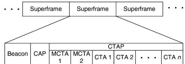
Fig. 3. IEEE 802.15.3 piconet superframes.
