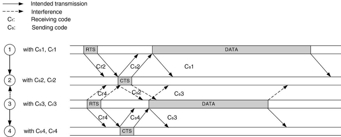
Fig. 6. MACA/R-T protocol [41].
