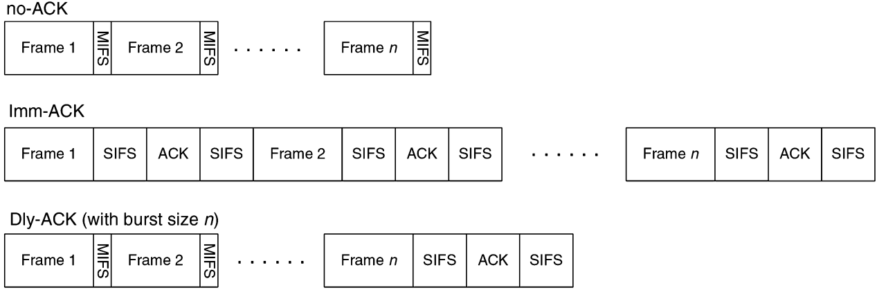
Fig. 7. No-ACK, Imm-ACK, and Dly-ACK mechanisms in IEEE 802.15.3.
