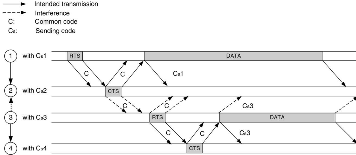
Fig. 5. MACA/C-T protocol [41].
