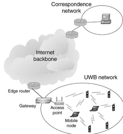
Fig. 1. UWB network architecture.
