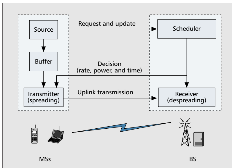
■ Figure 1. The centralized scheduler for the uplink transmission.
