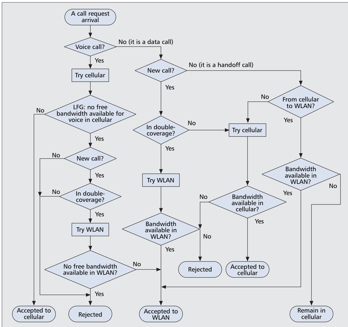
■ Figure 3. Call admission procedure for cellular/WLAN interworking.
