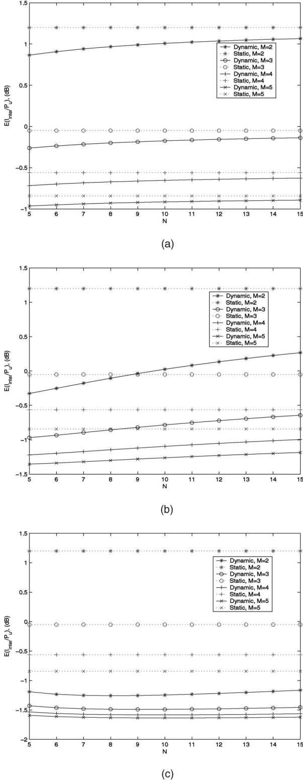
Fig. 3. E(I/P_U) for different number of resolvable paths under SW-CDGPS and DW-CDGPS. (a) \alpha = 1 . (b) \alpha = 10 . (c) \alpha = 100 .
