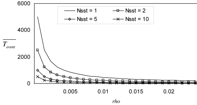
Figure 21 \overline{T}_{event} versus \rho for various values of N_{sst} at T_{active} = 10 , N_{hop} = 10 , T_{hop} = 1 and T_{sense} = 1
