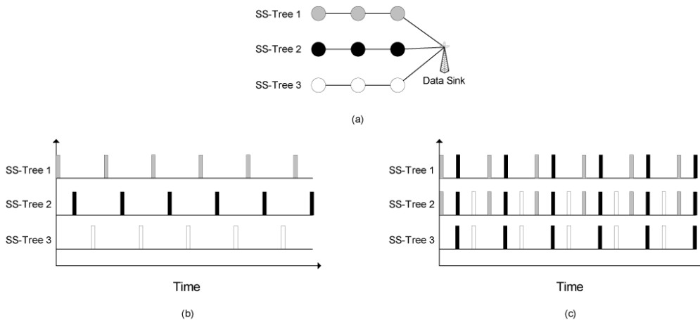
Figure 8 Impact of SS-Tree on spatial and temporal coverage: (a) SS-Tree assignment, (b) low duty cycle sleep scheduling and (c) event reporting windows
