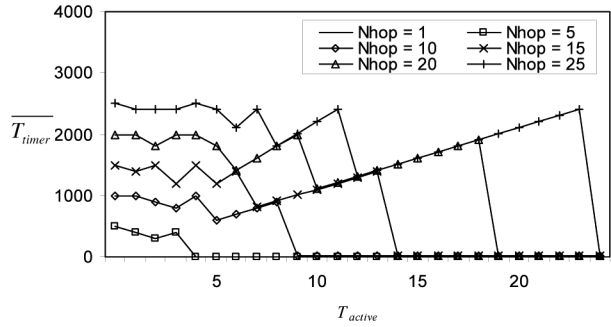
Figure 12 \overline{T}_{\text{timer}} versus T_{\text{active}} for various values of N_{\text{hop}} ( N_{\text{hop}} ) at \rho = 0.01 , T_{\text{hop}} = 1 and T_{\text{sense}} = 1
