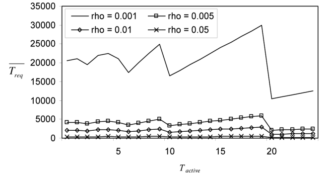
Figure 14 \overline{T}_{\text{req}} versus T_{\text{active}} for various values of \rho ( \rho ) at N_{\text{hop}} = 10 , T_{\text{hop}} = 1 and T_{\text{sense}} = 1
