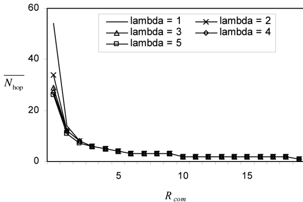
Figure 17 \overline{N}_{hop} versus R_{com} for various values of \lambda (lambda) at R_{sink} = 20
