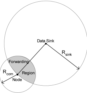
Figure 4 Forwarding region of a node in relationship to data sink
