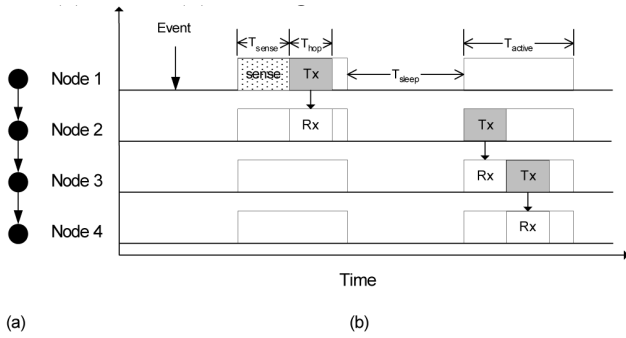
Figure 2 Event-driven data reporting timing: (a) route (b) timing
