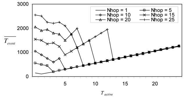
Figure 10 \overline{T}_{event} versus T_{active} for various values of N_{hop} ( N_{hop} ) at \rho = 0.01 , T_{hop} = 1 and T_{sense} = 1
