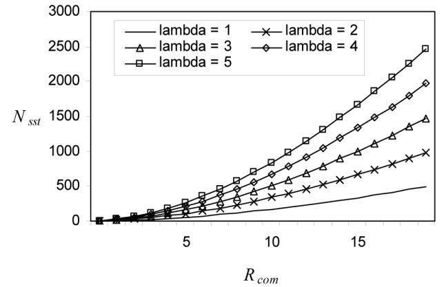
Figure 19 N_{sst} versus R_{com} for various values of \lambda (lambda) at R_{sink} = 20
