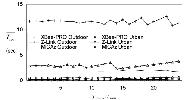
Figure 24 \overline{T_{\text{req}}} versus T_{\text{active}}/T_{\text{hop}} for different transceivers at different transmission ranges
