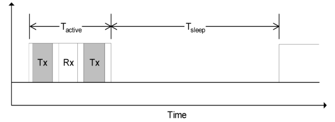
Figure 6 Example of transceiver activity in sleep scheduling
