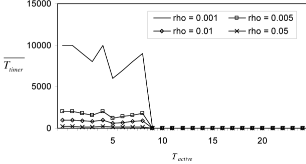
Figure 11 \overline{T}_{\text{timer}} versus T_{\text{active}} for various values of \rho ( \rho ) at N_{\text{hop}} = 10 , T_{\text{hop}} = 1 and T_{\text{sense}} = 1
