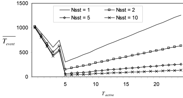
Figure 20 \overline{T}_{event} versus T_{active} for various values of N_{sst} at \rho = 0.01 , N_{hop} = 10 , T_{hop} = 1 and T_{sense} = 1
