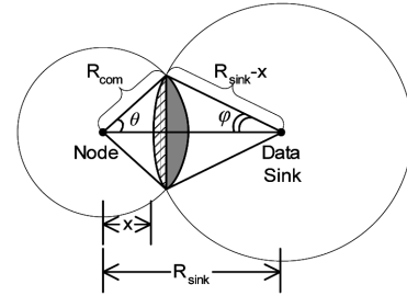
Figure 5 Geometric relationships for calculating expected N_{\text{hop}} per node
