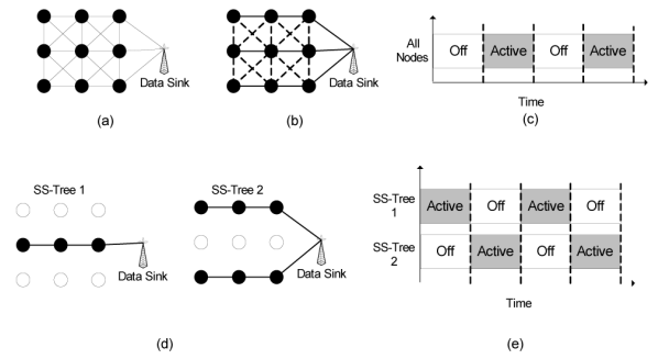
Figure 7 SS-Tree concept (a) WSN topology, (b) logical spanning tree overlay, (c) global sleep schedule, (d) SS-Tree configuration and (e) interleaved sleep schedules
