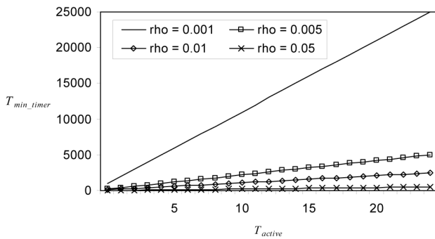
Figure 13 T_{\text{min\_timer}} versus T_{\text{active}} for various values of \rho ( \rho )
