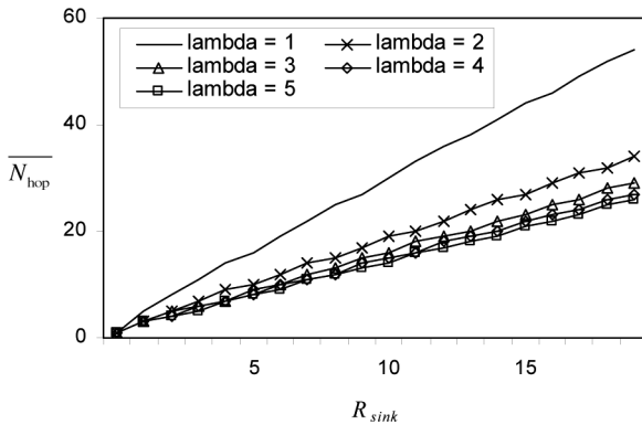
Figure 16 \overline{N}_{hop} versus R_{sink} for various values of \lambda (lambda) at R_{com} = 1
