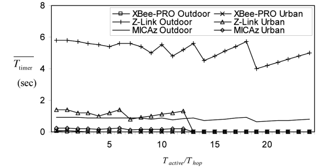
Figure 23 \overline{T_{\text{timer}}} versus T_{\text{active}}/T_{\text{hop}} for different transceivers at different transmission ranges
