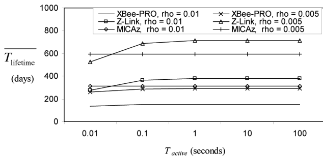
Figure 25 \overline{T}_{\text{lifetime}} versus T_{\text{active}} for the three different transceivers under different duty cycles
