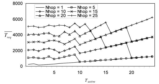
Figure 15 \overline{T}_{\text{req}} versus T_{\text{active}} for various values of N_{\text{hop}} ( N_{\text{hop}} ) at \rho = 0.01 , T_{\text{hop}} = 1 and T_{\text{sense}} = 1
