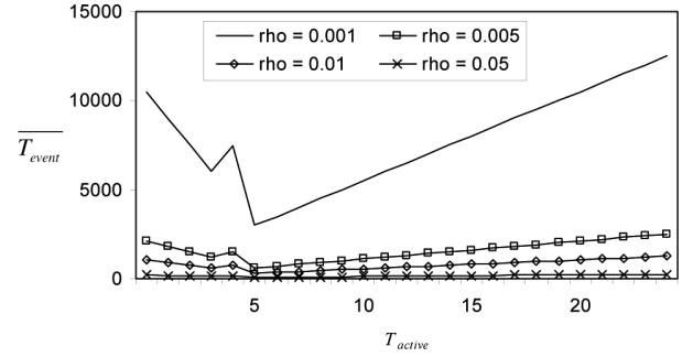
Figure 9 \overline{T}_{event} versus T_{active} for various values of \rho (rho) at N_{hop} = 10 , T_{hop} = 1 and T_{sense} = 1
