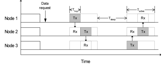
Figure 3 Request-driven data reporting timing
