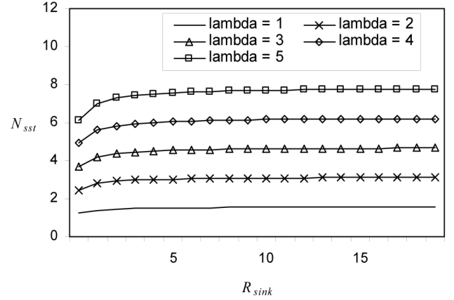
Figure 18 N_{sst} versus R_{sink} for various values of \lambda (lambda) at R_{com} = 1
