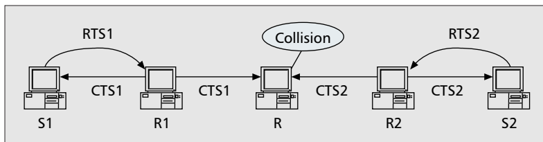
■ Figure 5. CTS collision.
