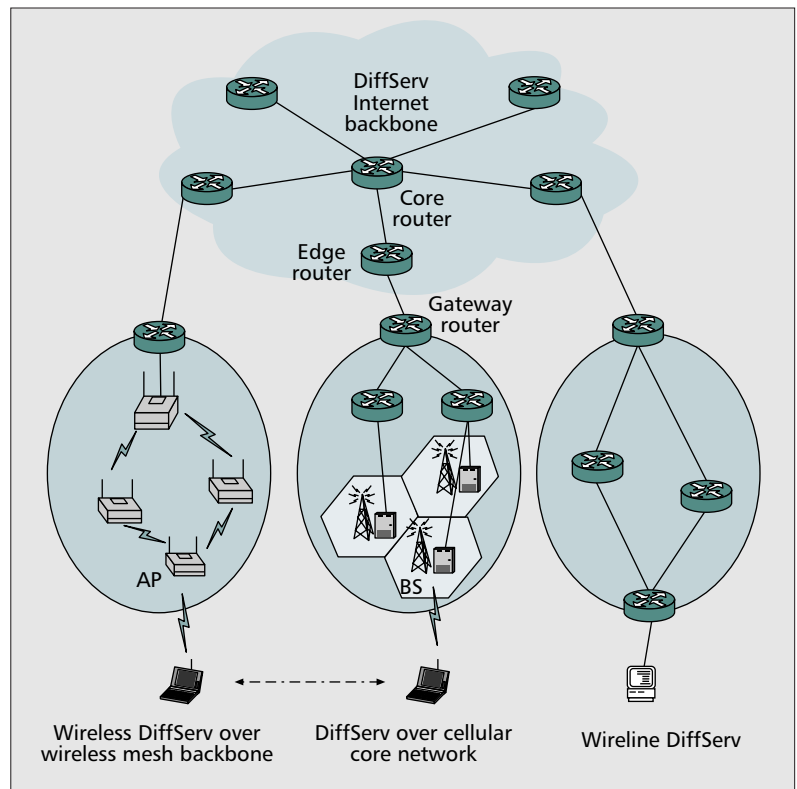
■ Figure 2. A DiffServ platform for network interconnection.
