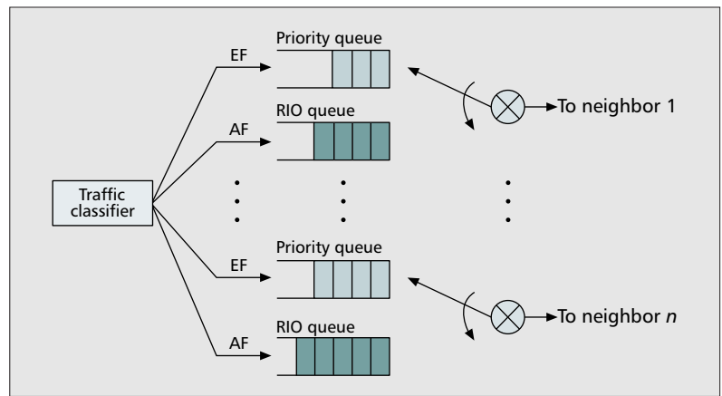
■ Figure 4. The service differentiation mechanism within a wireless router.
