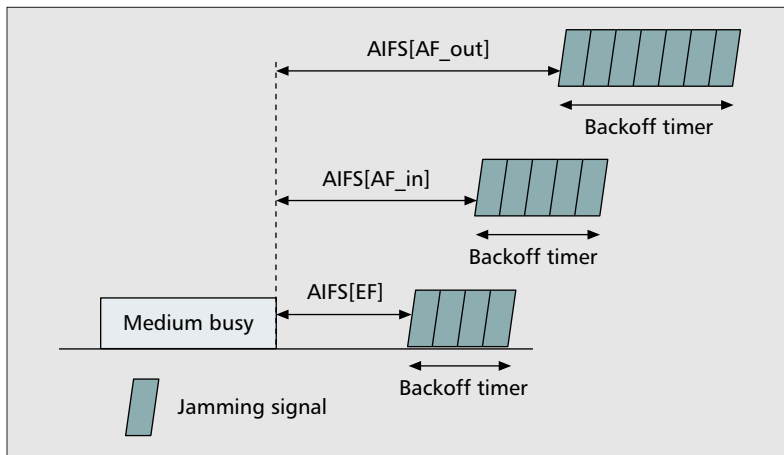
■ Figure 6. The black burst contention scheme.
