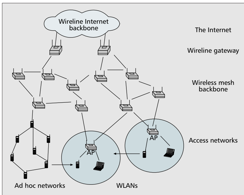
■ Figure 1. A network architecture for broadband wireless access.
