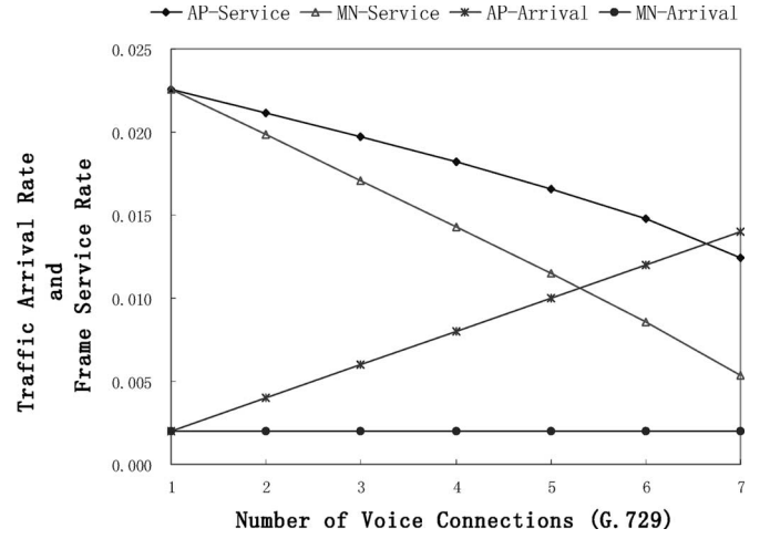
Fig. 3. Traffic arrival rate and frame service rate (802.11b).
