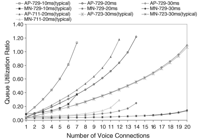
Fig. 4. Queue utilization ratio of the AP and MNs (802.11b).
