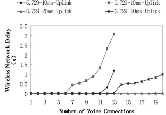
Fig. 6. Delay comparison between uplink and downlink voice flows.
