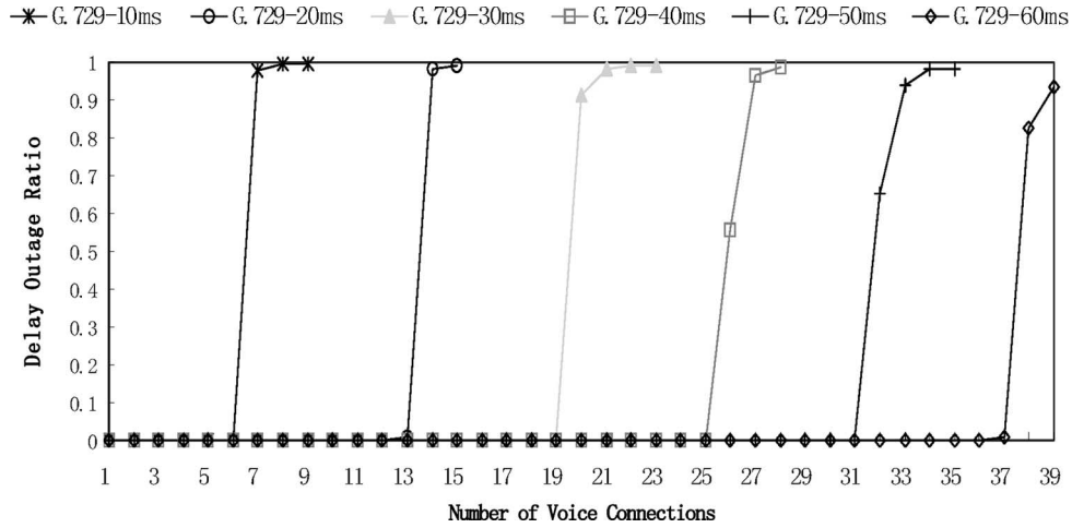
Fig. 7. Delay outage ratio of voice traffic.
