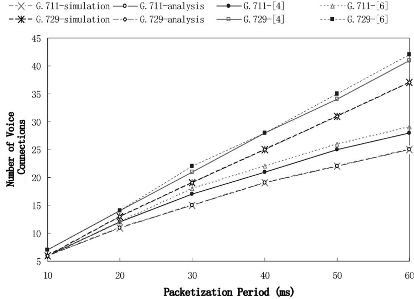
Fig. 8. Maximum number of voice connections.
