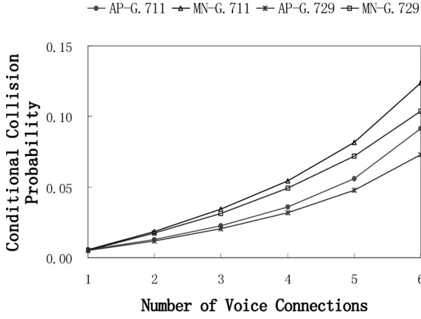
Fig. 2. Comparison of the conditional collision probabilities of the AP and MNs (802.11b).
