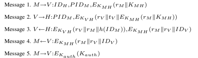
Fig. 2. Authentication Protocol I for Roaming Services
