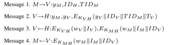
Fig. 5. Authentication Protocol II for Roaming Services
