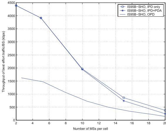
Fig. 6. Throughput of best effort traffic using the IS95B-SHO scheme
