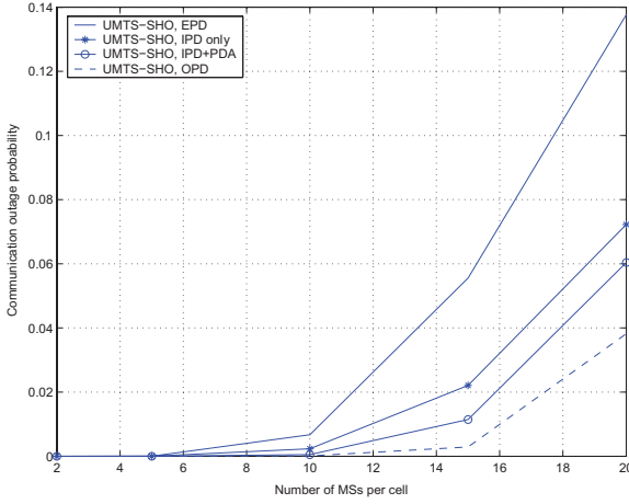
Fig. 3. Outage probability using the UMTS-SHO scheme
