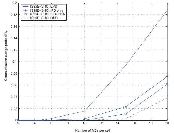
Fig. 2. Outage probability using the IS95B-SHO scheme
