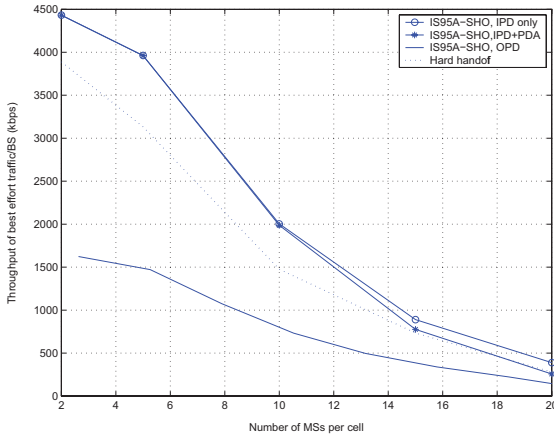
Fig. 5. Throughput of best effort traffic using the IS95A-SHO scheme
