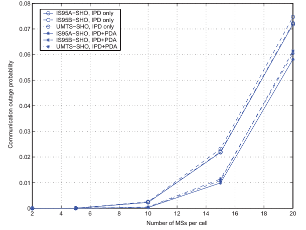
Fig. 4. Outage probability using the proposed power distribution scheme
