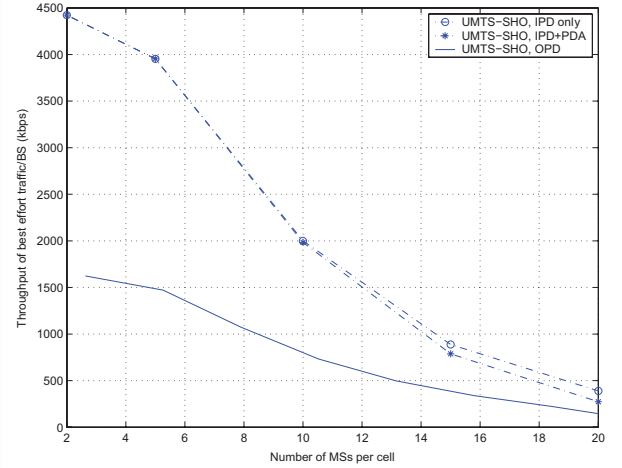
Fig. 7. Throughput of best effort traffic using the UMTS-SHO scheme
