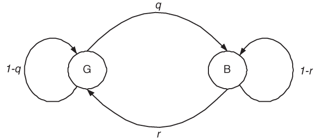
Fig. 3. Markov model for frame success/failure process over wireless fading channels.
