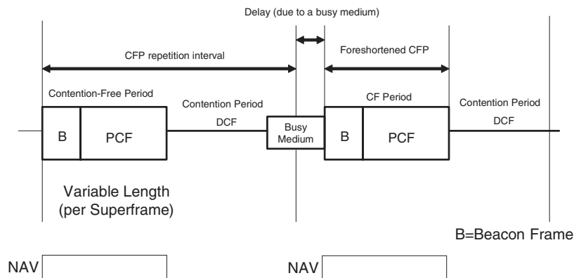
Figure 4. PCF stretch effect.
