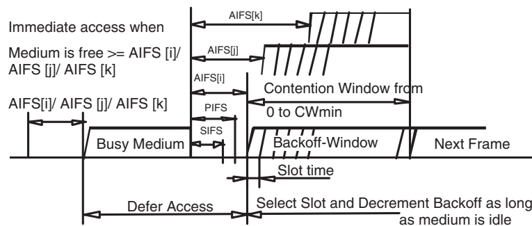
Figure 5. Enhanced distributed Co-ordination function.
