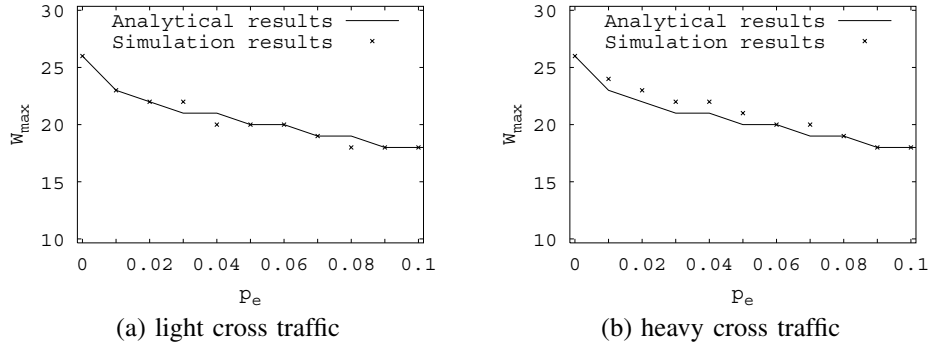
Fig. 6. Maximum rwnd to guarantee delay outage probability.
