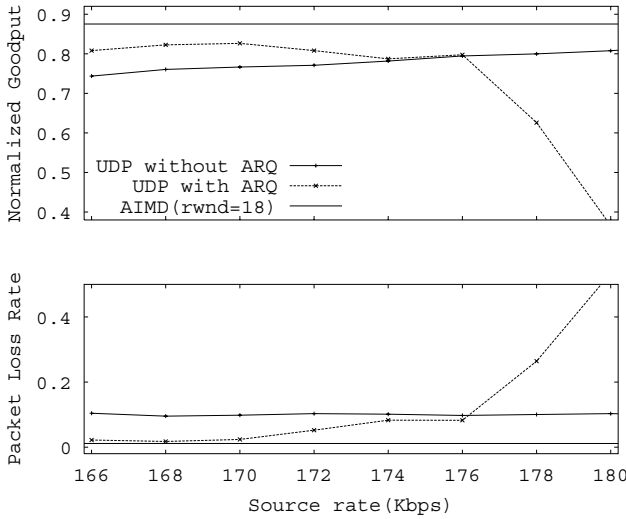
Fig. 11. AIMD vs. UDP, p_e = 0.1
