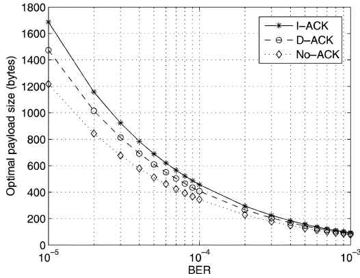
Fig. 7. Optimal payload size versus BER in CTA.
