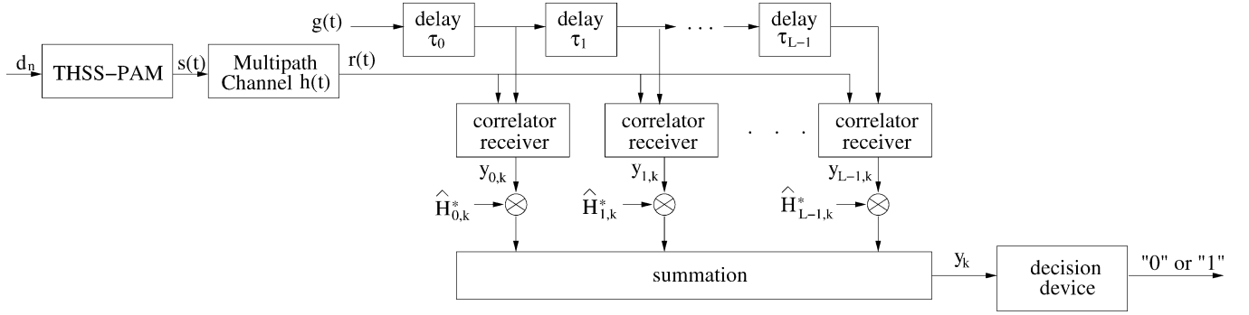
Fig. 1. Transceiver structure of the UWB system.
