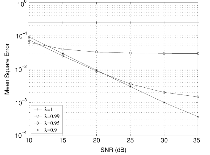
Fig. 4. Mean square error performance of the proposed H_\infty algorithm with NDFP = 0.1.
