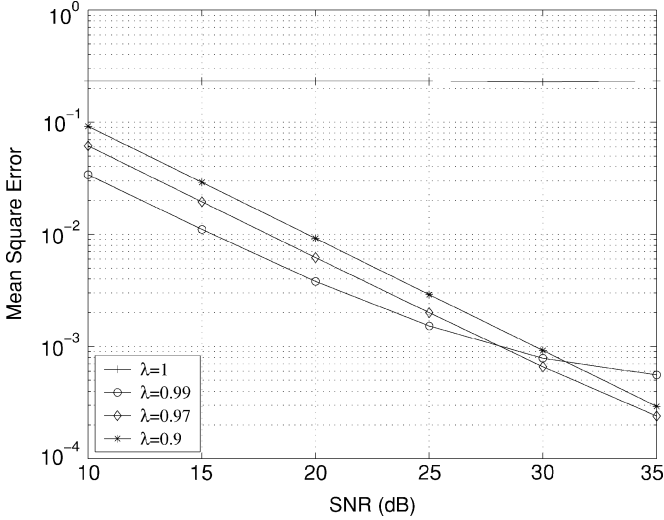
Fig. 3. Mean square error performance of the proposed H_\infty algorithm with NDFP = 0.01.
