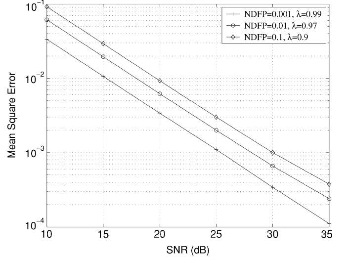
Fig. 5. Mean square error performance of the proposed H_\infty algorithm with different NDFPs and associated optimal forgetting factor \lambda .
