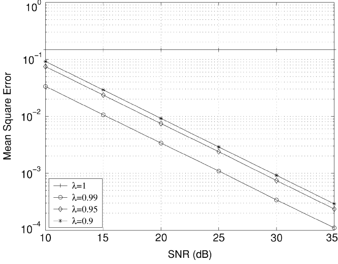
Fig. 2. Mean square error performance of the proposed H_\infty algorithm with NDFP = 0.001.
