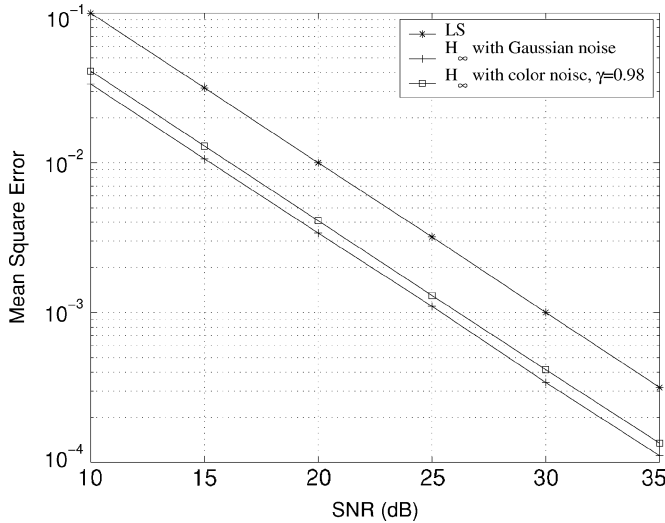
Fig. 7. Mean square error performance of the proposed H_\infty algorithm under colored noise.
