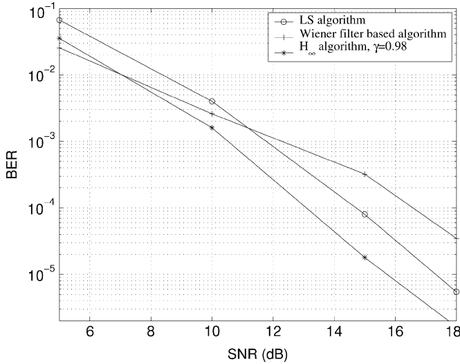
Fig. 6. BER performance of the proposed H_\infty , the LS, and the Wiener filter-based algorithms.
