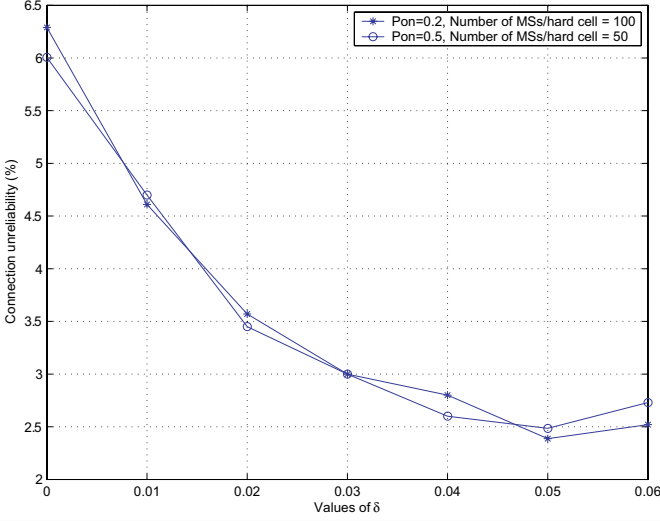
Fig. 8. Effect of values of \delta on connection unreliability.
