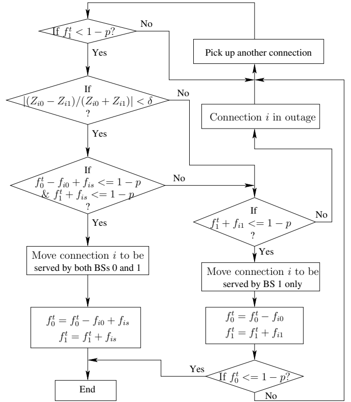
Fig. 2. Power re-distribution flow chart.
