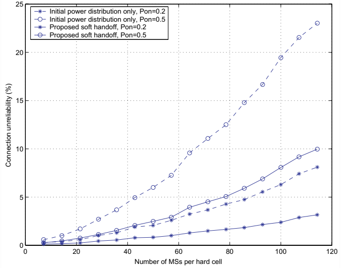
Fig. 6. Comparison between the proposed SHO scheme and the scheme with initial power allocation only.
