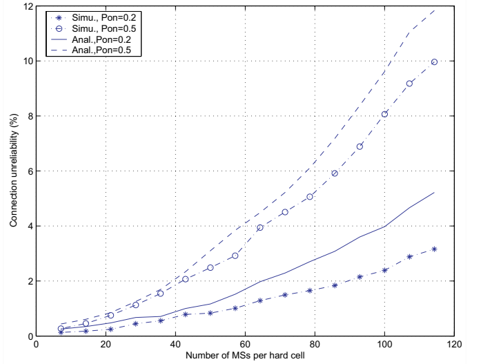
Fig. 3. Performance of the proposed SHO scheme.
