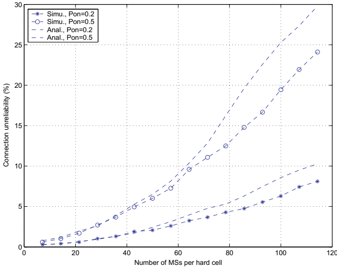
Fig. 4. Performance of the soft handoff with initial power allocation only.
