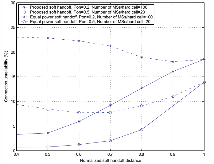
Fig. 7. Comparison between the proposed SHO scheme and the equal power soft handoff scheme.
