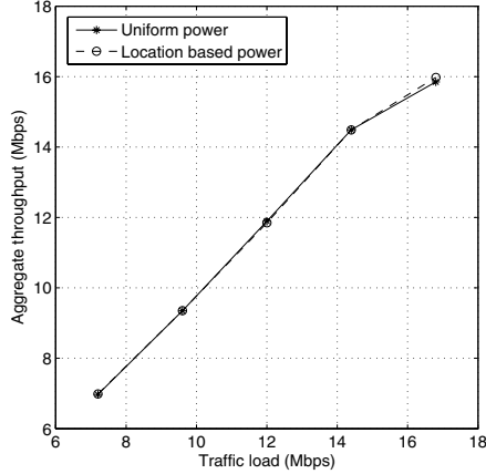
Fig. 6. Aggregate throughput of the uniform power and location based power allocation strategies in the two-cluster topology.
