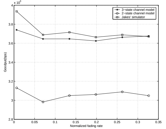
Fig. 4. The accuracy of three-state Markov channel model.
