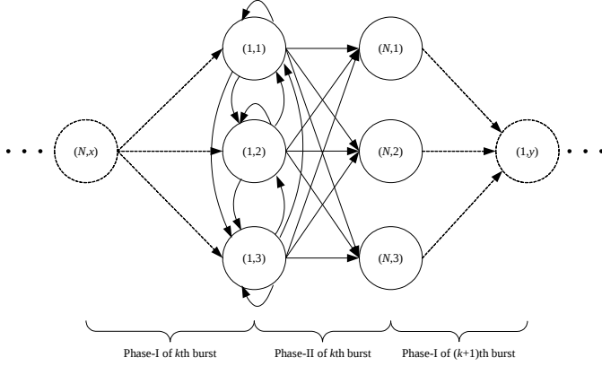
Fig. 3. State transition diagram of phase-II transmission process. N is the burst size. Note that the transition probability from state \{(N, 1), (N, 2), (N, 3)\} to state (1, y) is one.
