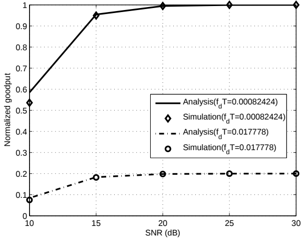
Fig. 10. Normalized goodput versus SNR for f_dT = 0.00008 and 0.01778 .
