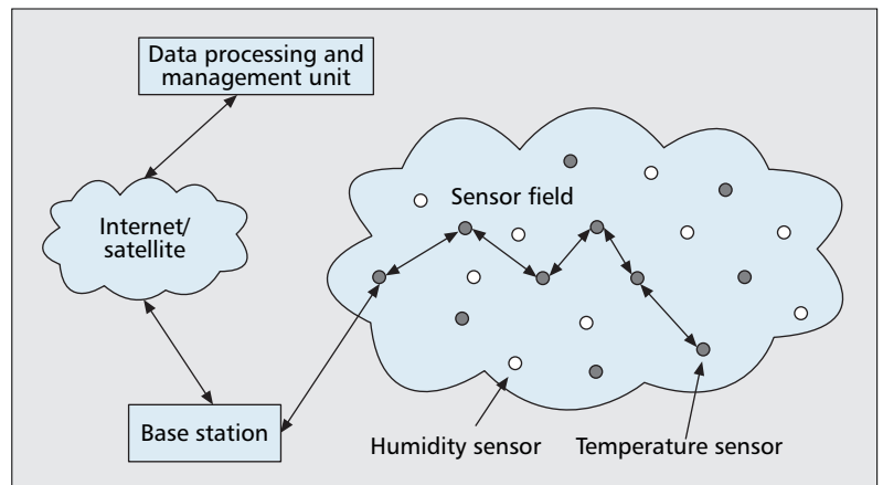
■ Figure 1. The architecture of a wireless sensor network.
