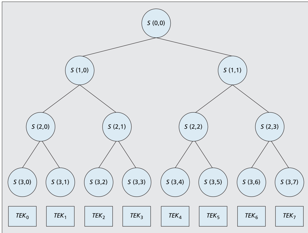
■ Figure 3. Example of a hash binary tree with D = 3 .
