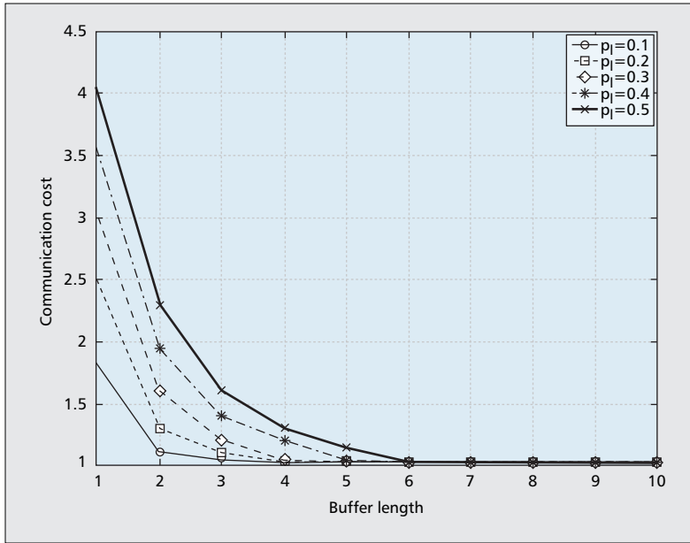
■ Figure 5. Normalized communication costs vs. key buffer length.
