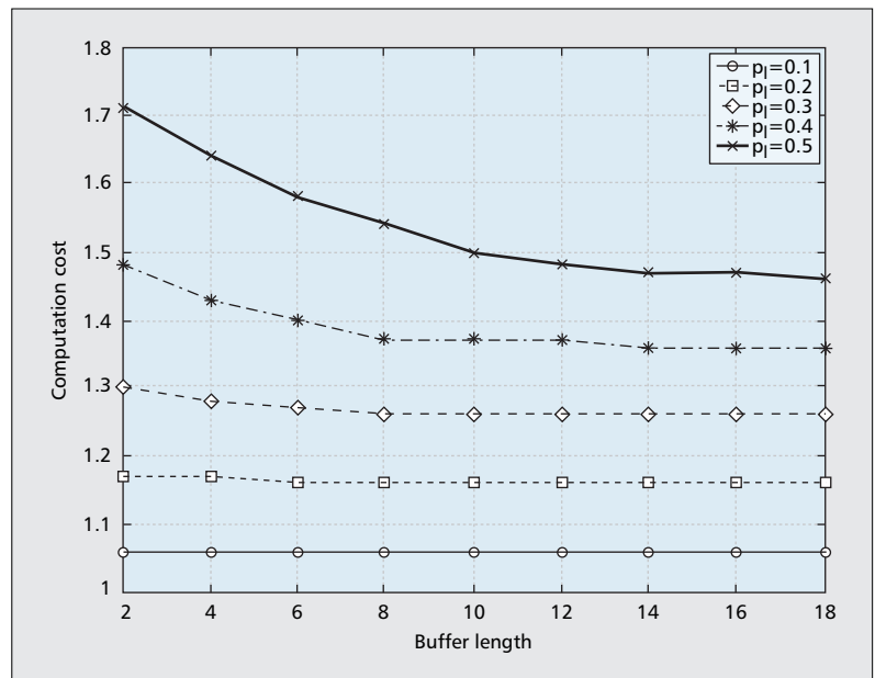
Figure 6. Computation costs vs. key buffer length.
