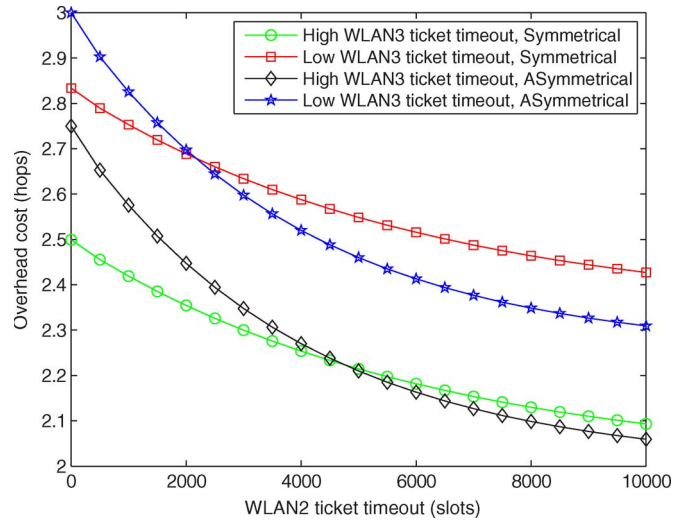
Fig. 8. Overhead cost versus WLAN2 ticket timeout for the high and low WLAN3 ticket timeouts.
