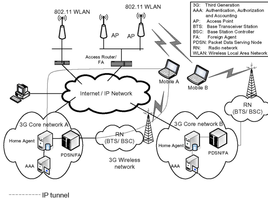
Fig. 1. Loosely coupled 802.11 WLAN and 3G cellular networks.
