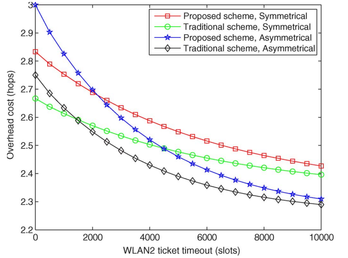
Fig. 7. Overhead cost versus WLAN2 ticket timeout for the proposed and traditional schemes.
