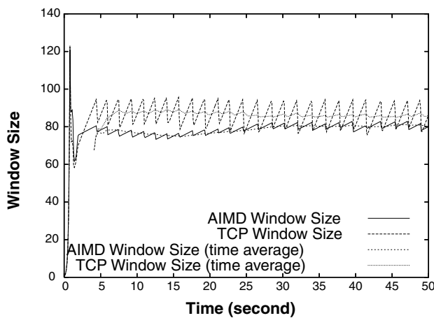
(b) Window trace
