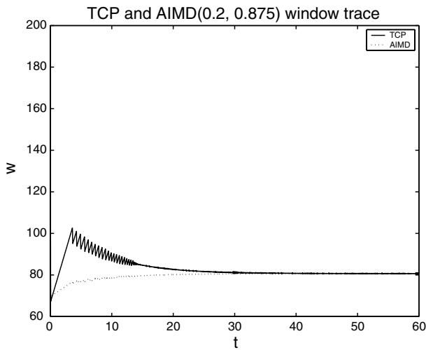
(a) TCP and AIMD(0.2, 0.875) window trace
