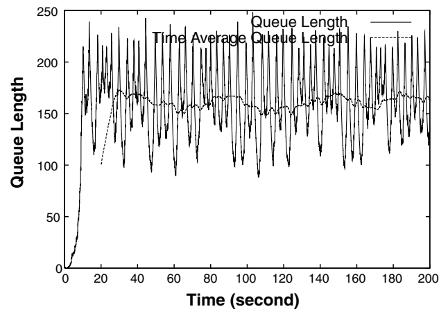
Fig. 14. Multiple-bottleneck, heterogeneous round-trip delays.
