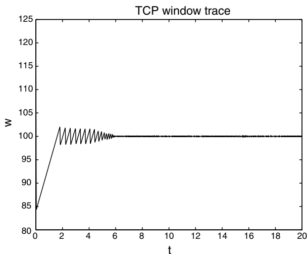
(a) TCP window trace
