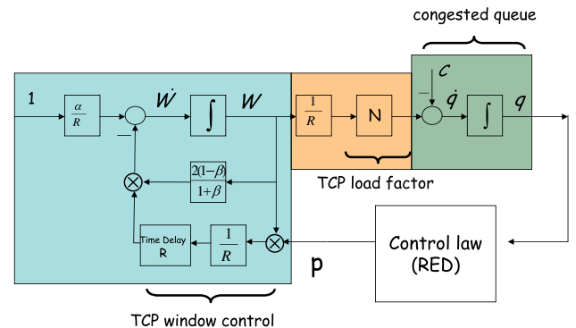
Fig. 1. Block diagram of generalized AIMD/RED system.
