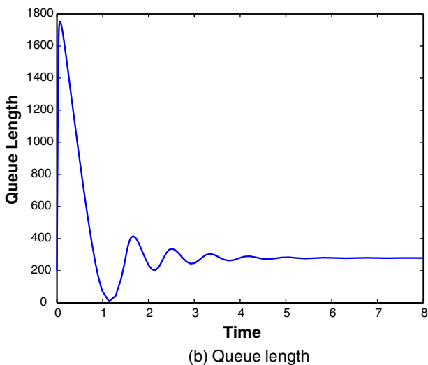
Fig. 6. AIMD(0.2, 0.875) flows.
