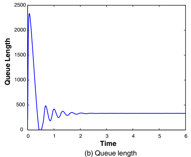
Fig. 7. TCP vs. AIMD(0.2, 0.875) flows.
