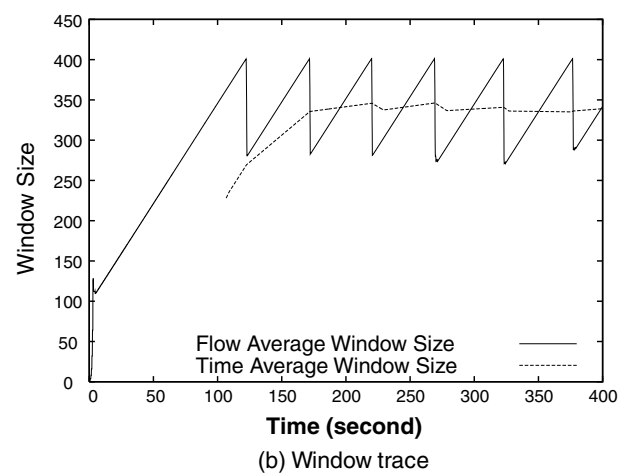
Fig. 11. TCP, K_p = 0.0001 , R = 400 ms.
