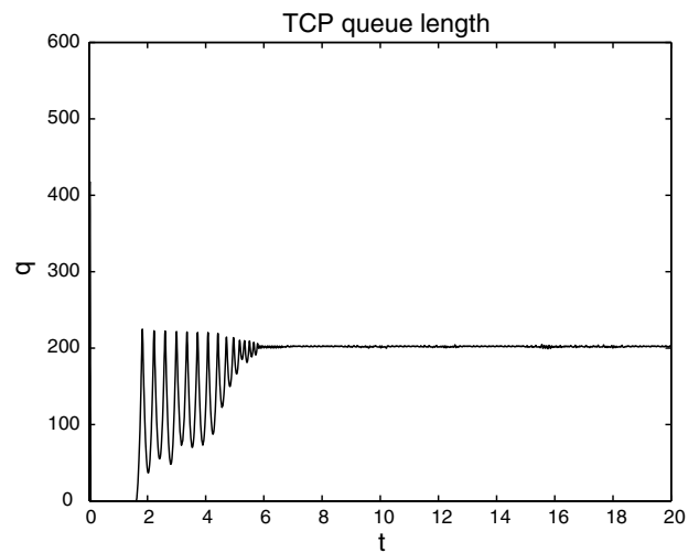
(a) TCP queue length
