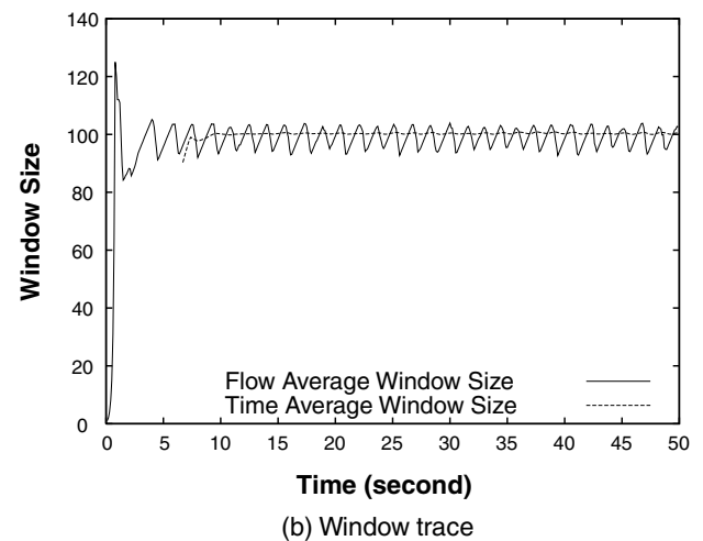
Fig. 9. TCP, K_p = 0.00002 , R = 100 ms.
