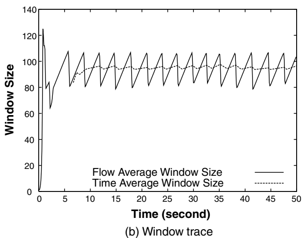
Fig. 8. TCP, K_p = 0.0001 , R = 100 ms.
