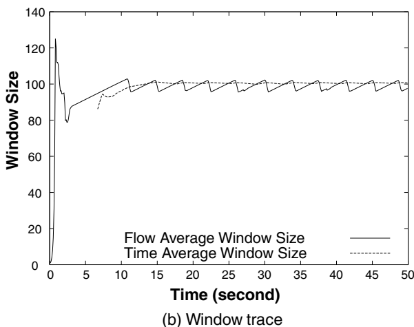
Fig. 10. AIMD(0.2,0.875), K_p = 0.0001 , R = 100 ms.
