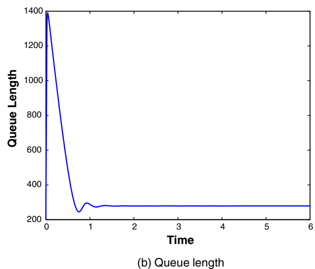
Fig. 5. TCP flows.
