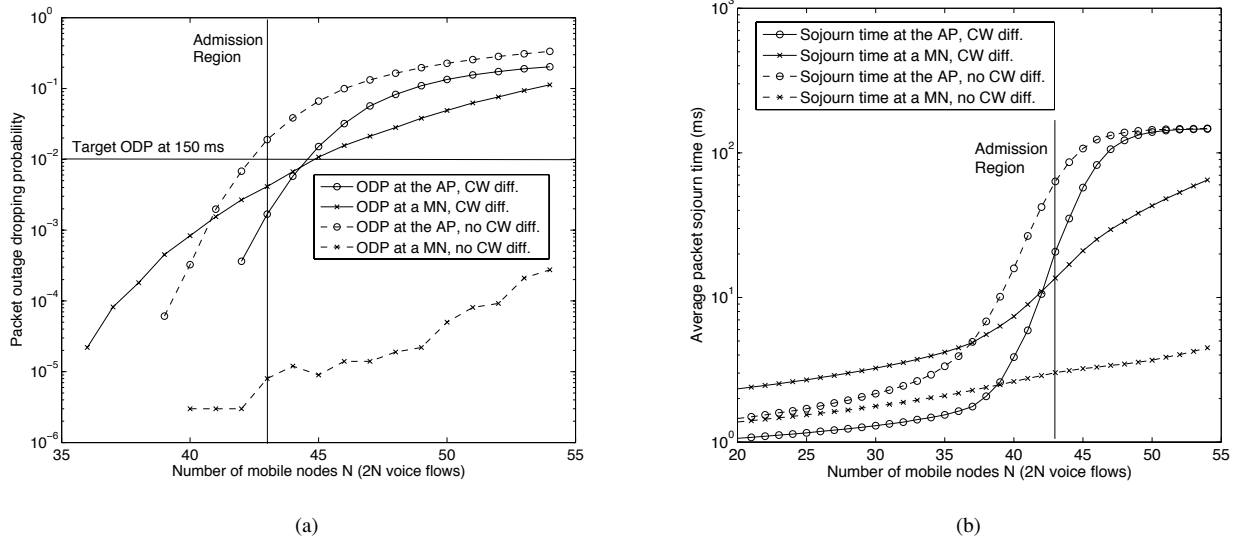
Fig. 4. The impact of the contention window on the QoS performance when downlink flows are aggregated at the AP, with p_{on} = 0.5 , d = 300 ms, and \epsilon = 0.01 . (a) Simulation results of the packet outage dropping probability. (b) Simulation results of the average packet sojourn time.
