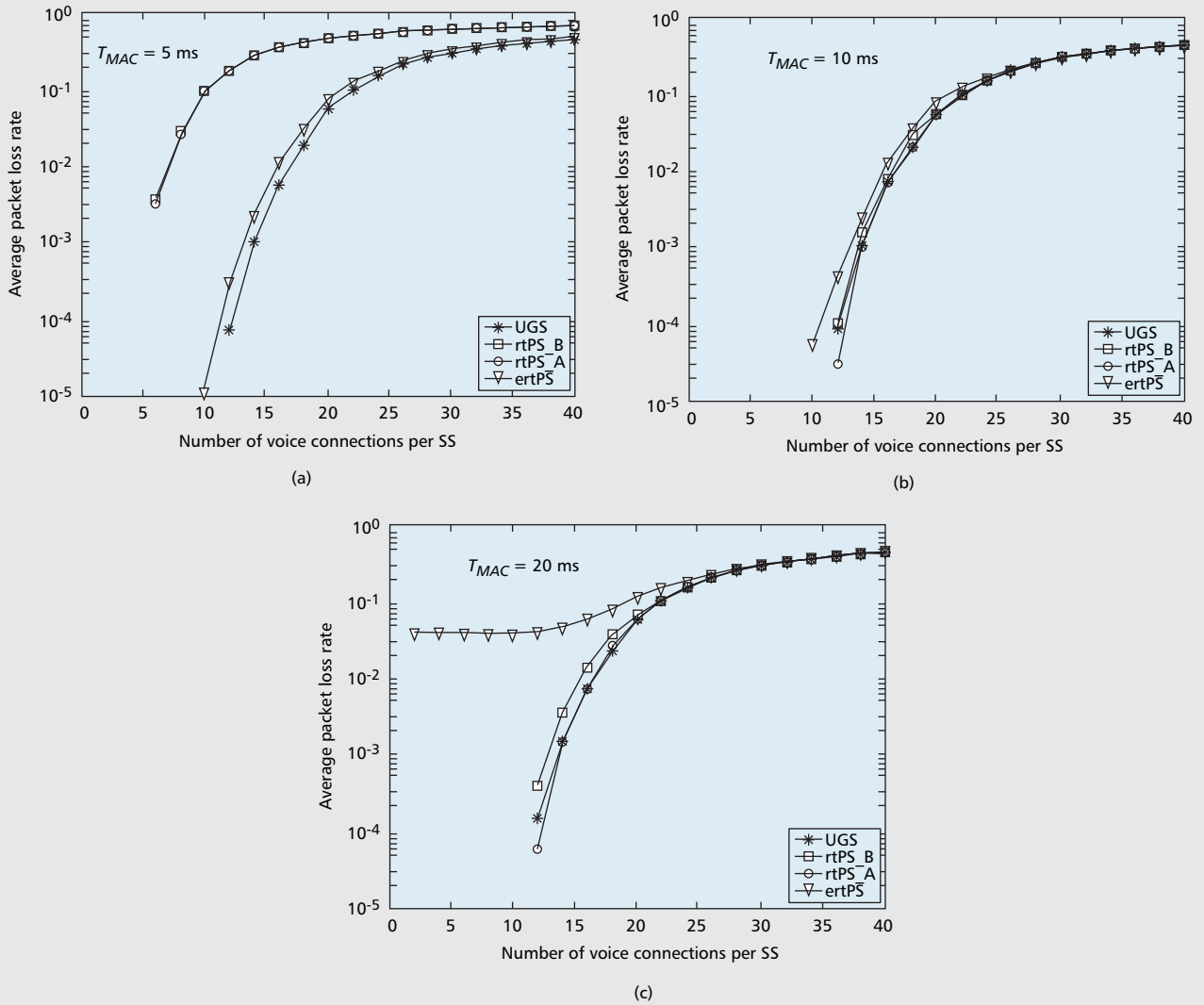
■ Figure 2. Average packet loss rate: a) T_{MAC} = 5 ms; b) T_{MAC} = 10 ms; c) T_{MAC} = 20 ms.
