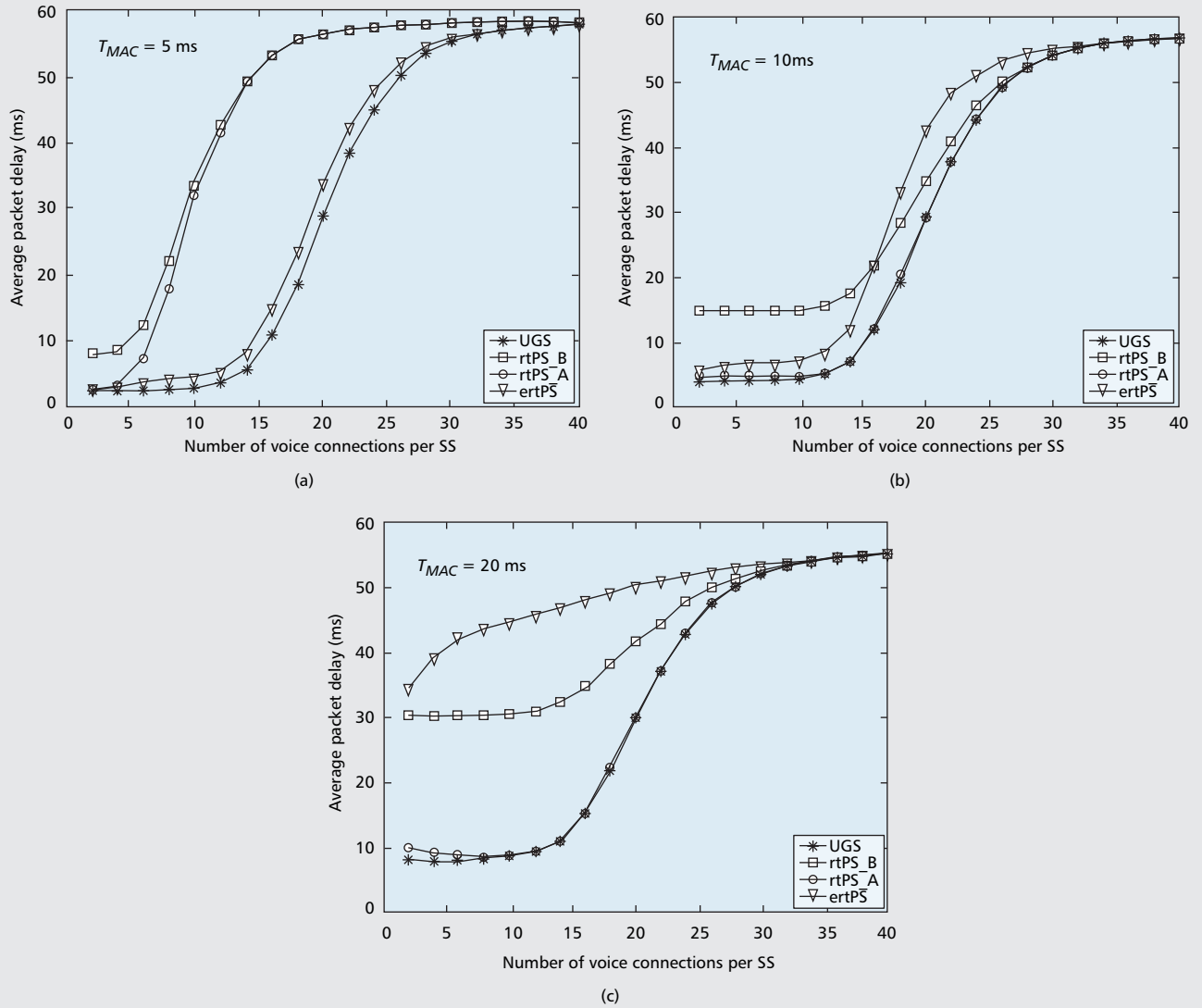
■ Figure 1. Average packet transmission delay: a) T_{MAC} = 5 ms; b) T_{MAC} = 10 ms; c) T_{MAC} = 20 ms.
