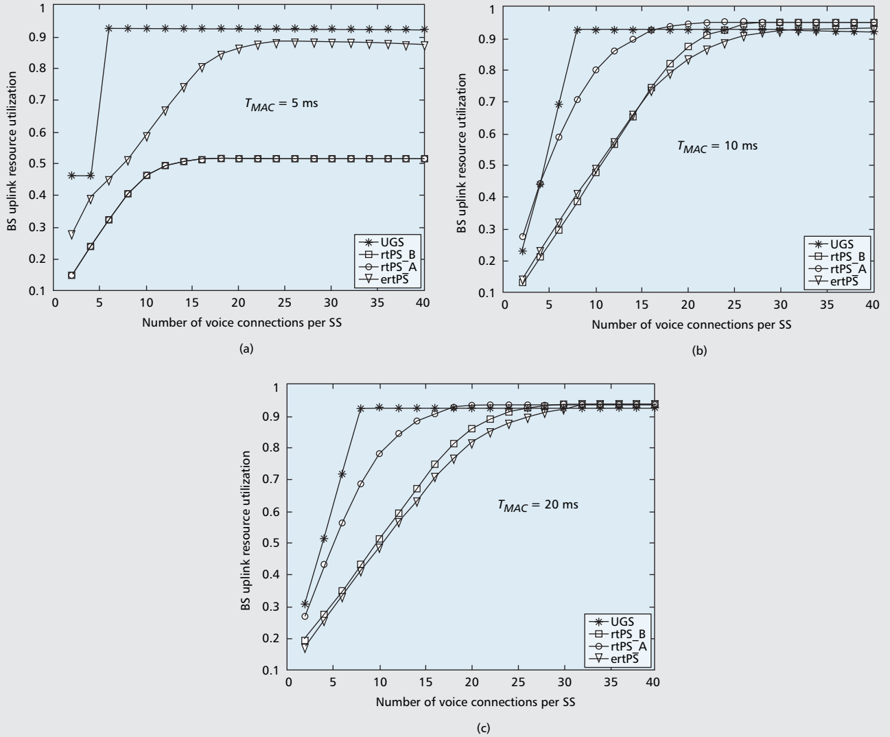
■ Figure 3. BS uplink resource utilization: a) T_{MAC} = 5 ms; b) T_{MAC} = 10 ms; c) T_{MAC} = 20 ms.
