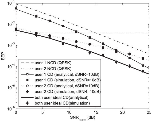
Fig. 2. Bit error performance of both users when SNR of user 2 is fixed at 15dB for differential SNR gain of 10 dB.
