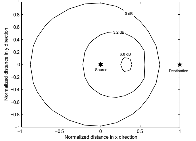
Fig. 5. Cooperative region of the proposed scheme for various SNR gain over direct transmission when P_e = 10^{-2} and \alpha = 3 (urban area).
