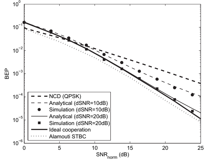
Fig. 3. Bit error performance of user 1 compared with Alamouti STBC scheme for similar channels towards the BS for various inter-user channel conditions.
