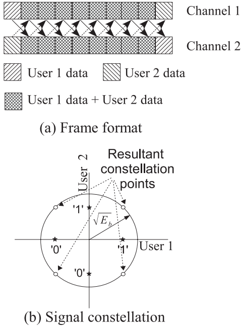
Fig. 1. Transmission frame format and the signal constellation of QPSK modulation.
