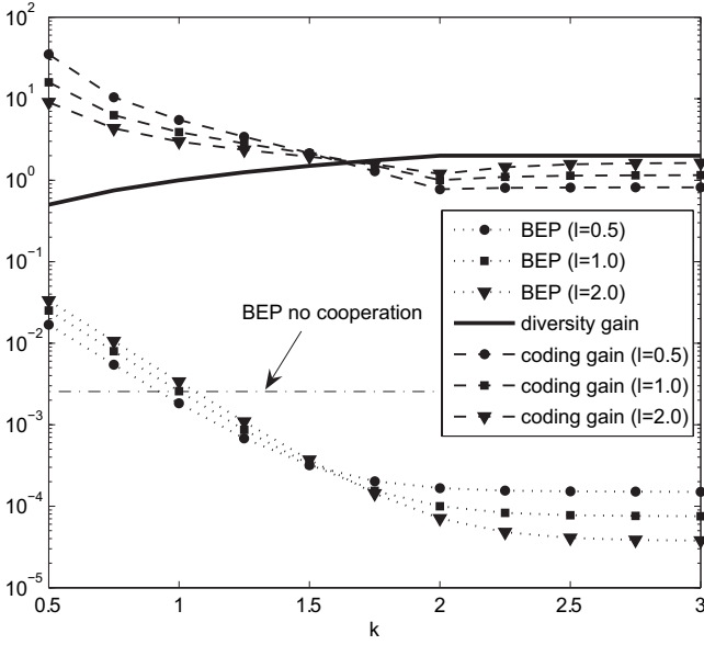
Fig. 4. BEP, coding gain and diversity gain provided by the scheme at high SNR for various inter-user and user 2 to BS channel conditions.
