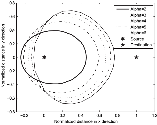
Fig. 6. Cooperative region of the proposed scheme for various path loss coefficient \alpha when P_e = 10^{-2} and G_{cdnorm} = 3.2dB .
