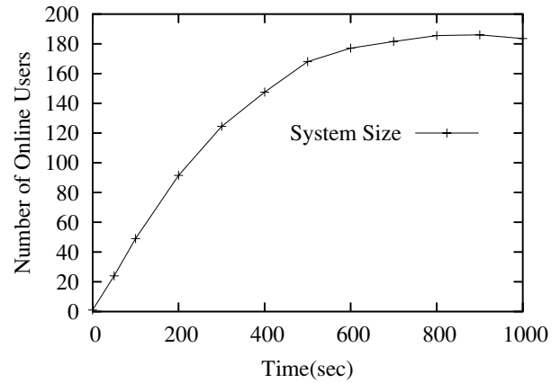
Fig. 15. System size during 1000-sec simulation.
