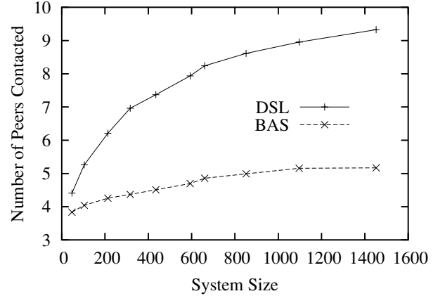
Fig. 12. Join/Search cost for DSL and BAS.
