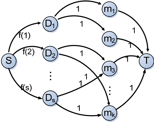
Fig. 9. Constructed flow network G .
