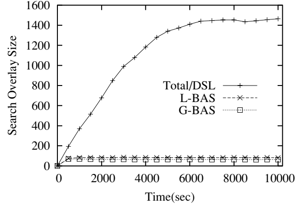
Fig. 11. The size of index structure.
