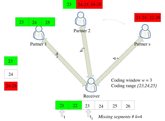
Fig. 7. Analysis of CW assignment problem.
