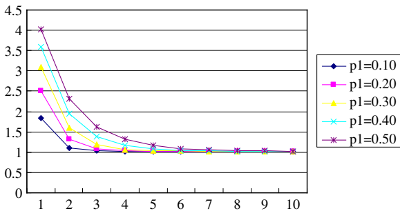
Fig. 6. Normalized communication costs C_{\text{comm}} vs. the key buffer length t ( n = 500 , \alpha = 10 ).
