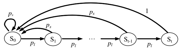
Fig. 5. State transition diagram of each group user.
