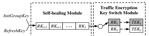
Fig. 2. Self-healing group key distribution with time-limited node revocation.
