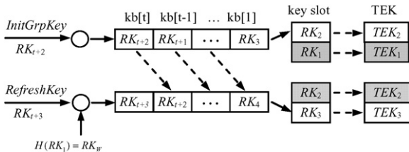
Fig. 3. Initial setup and TEK refreshment.
