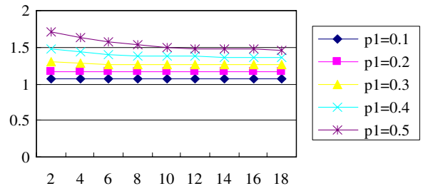
Fig. 7. Computation costs of node vs. key buffer length t ( n = 500 ).
