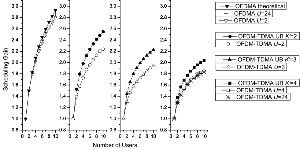
Fig. 4. Scheduling gain of OFDMA and OFDM-TDMA systems with different number of chunks in use.
