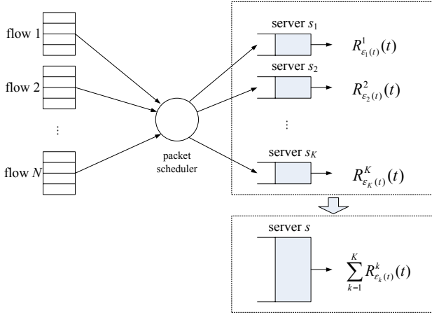
Fig. 1. Queueing model for multi-user scheduling in the OFDM system.
