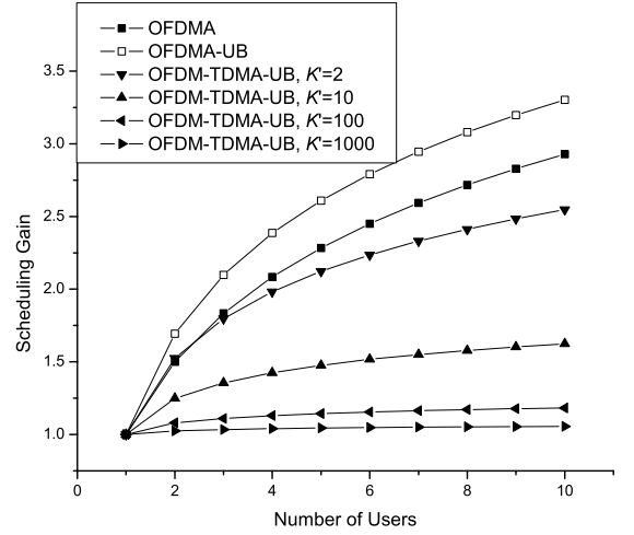
Fig. 2. Theoretical scheduling gain of OFDMA and OFDM-TDMA systems.
