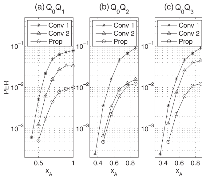
Fig. 7. Coded PER along different paths when the average SNR per BS at the three-cell boundary is set to 3.5 dB in the PA channel model with N_T = 1 .
