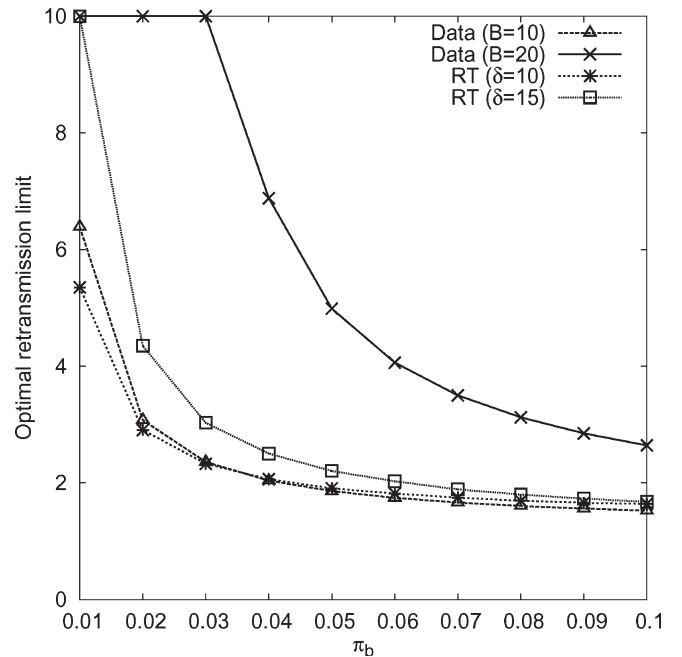
Fig. 2. Optimal retransmission limit ( MAX = 10 ).
