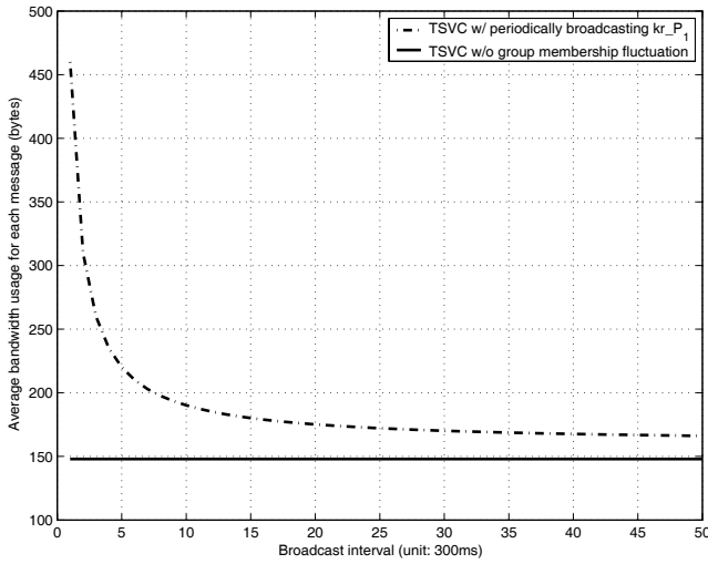
Fig. 6. Average bandwidth usage of different broadcast intervals
