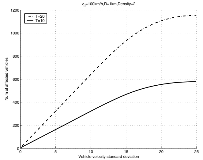
Fig. 7. Affected vehicles due to vehicle velocity standard deviation
