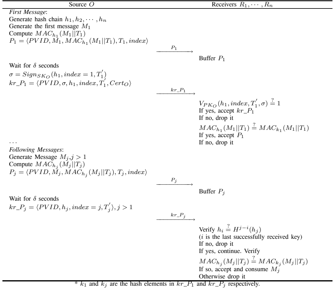
Fig. 4. The proposed security scheme
