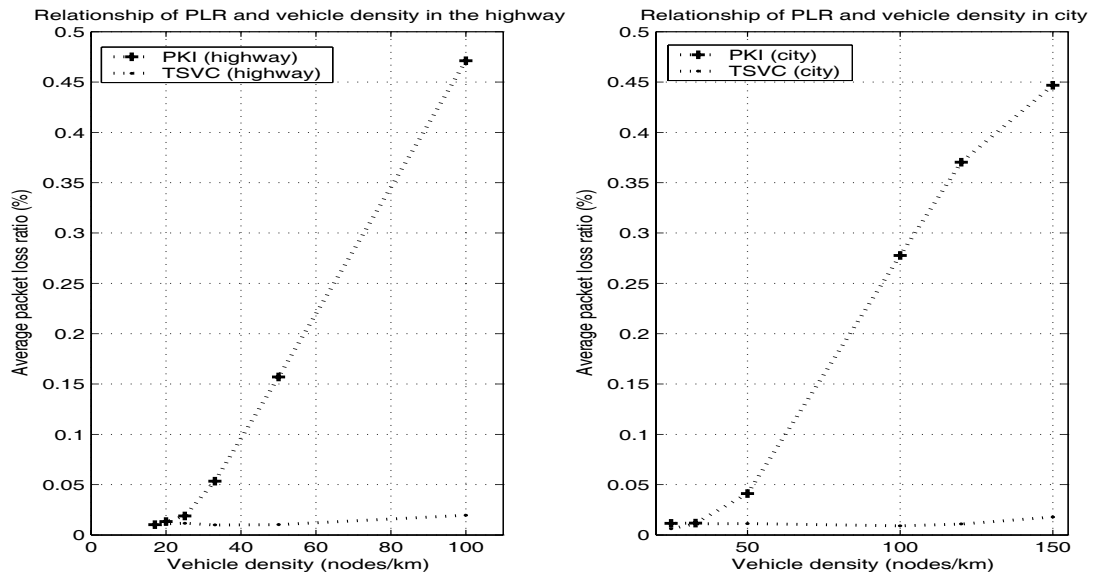
Fig. 11. Relationship of PLR and vehicle density
