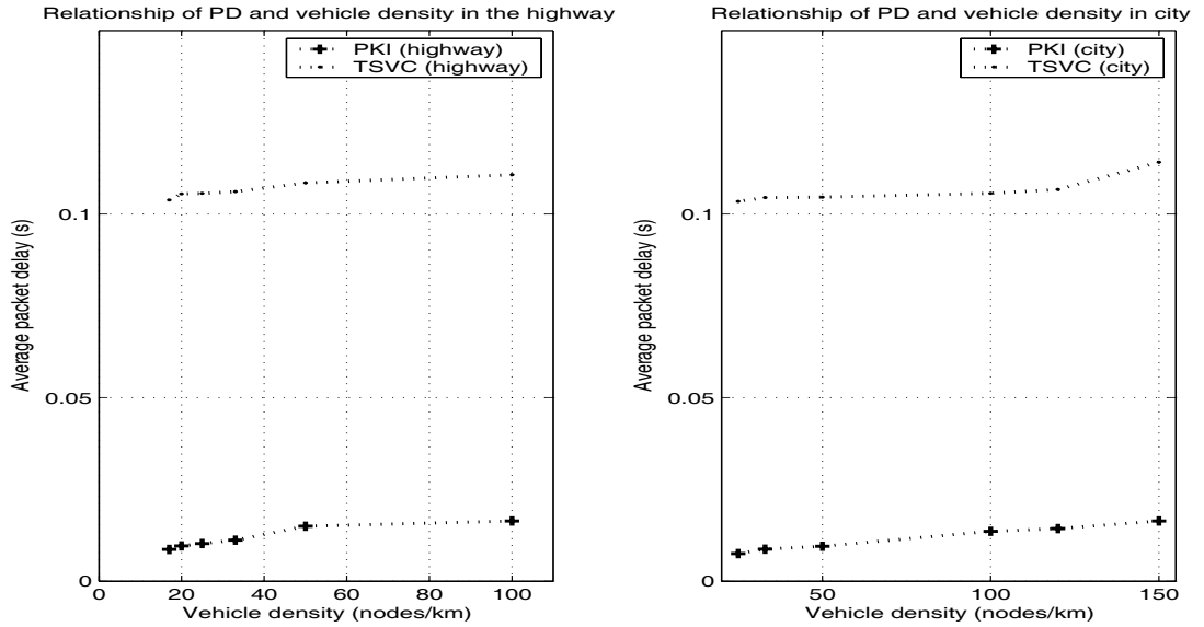
Fig. 10. Relationship of PD and vehicle density
