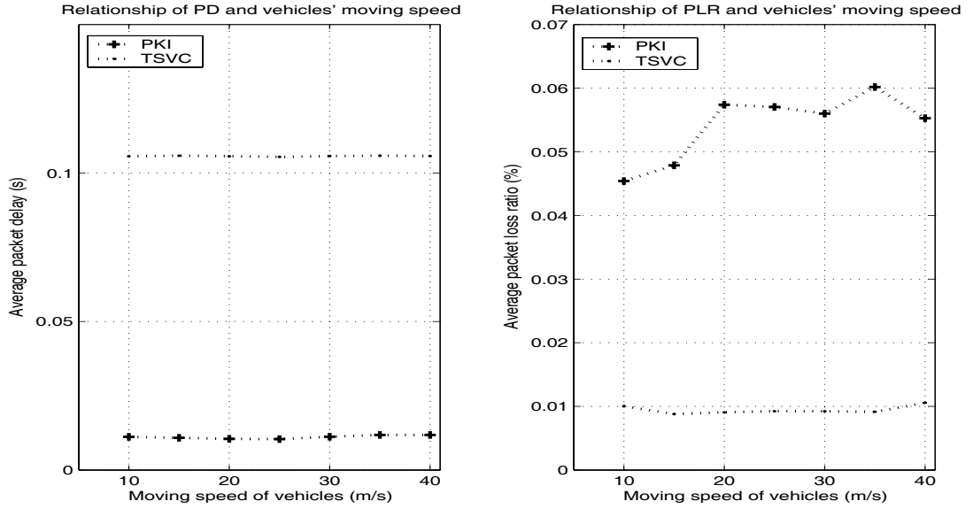
Fig. 9. Impact of vehicles' moving speed
