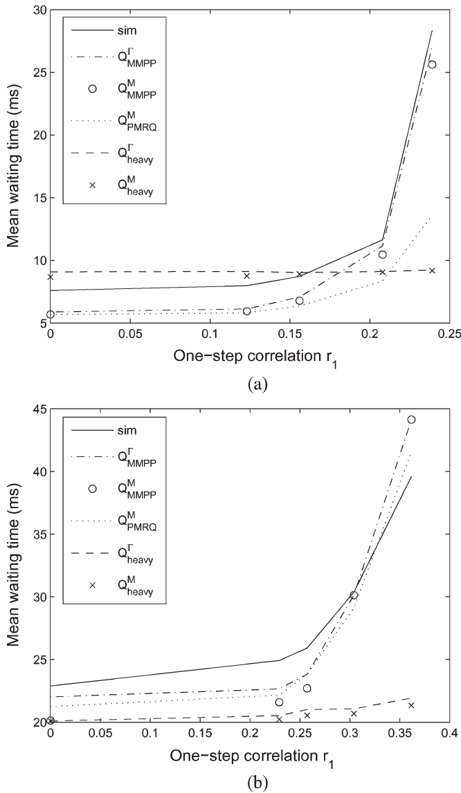
Fig. 2. Comparisons of mean waiting time obtained from simulations and from the approximated queuing systems (listed in Table I) in different degrees of burstiness, with \lambda_a = 0.6 , and M = 2 . (a) Low bursty traffic c^2 = 2 . (b) High bursty traffic c^2 = 10 .
