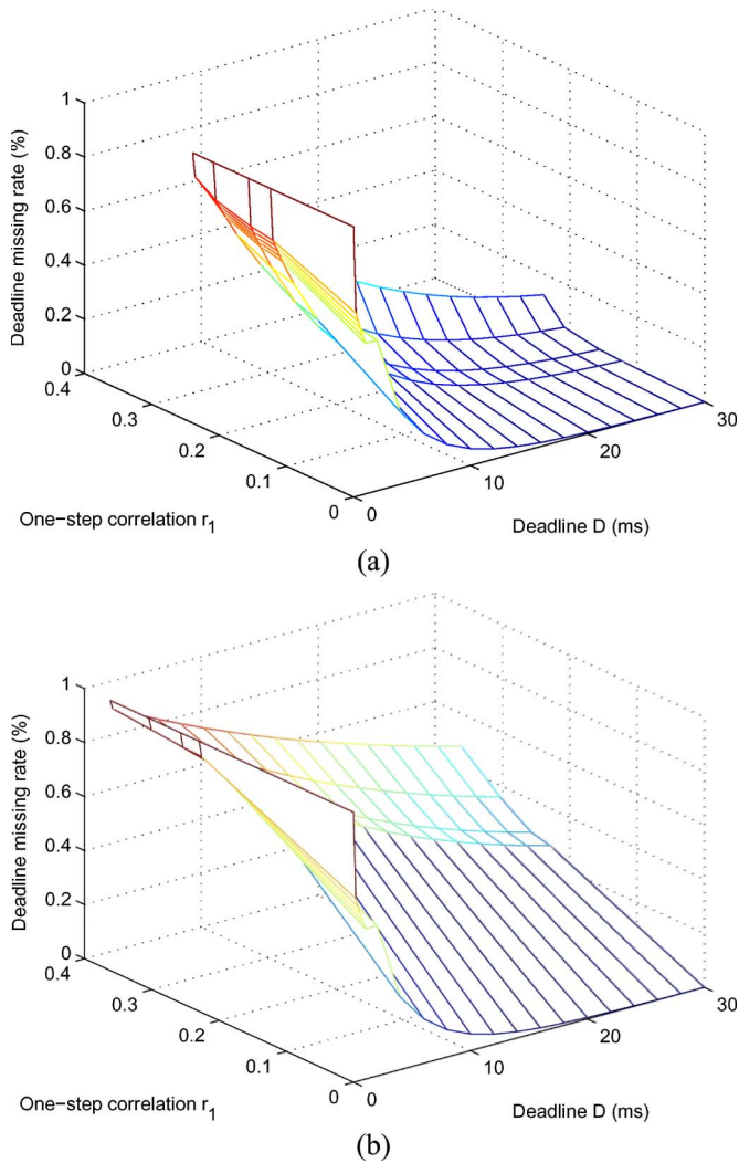
Fig. 5. Dead line rate (DMR) versus one-step correlation ( r_1 ) for different degrees of burstiness, with N_1 = N_2 = 5 , M = 2 , and \lambda_a = 0.6 . (a) Low bursty traffic c^2 = 2 . (b) High bursty traffic c^2 = 10 .
