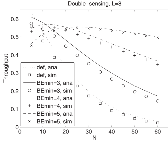
Fig. 3. Saturation throughput
