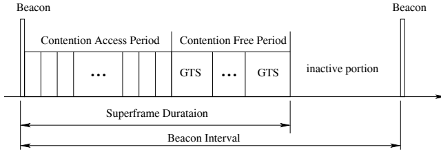
Fig. 1. IEEE 802.15.4 superframe structure in the beacon-enabled mode
