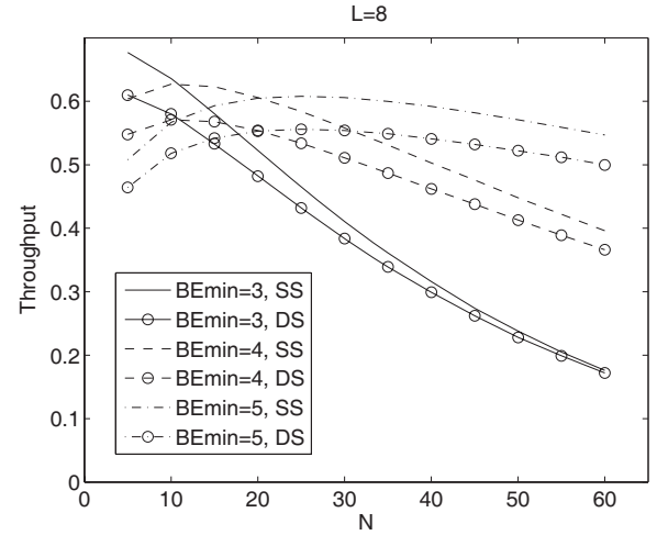
Fig. 7. Saturation throughput comparison between SS and DS modes
