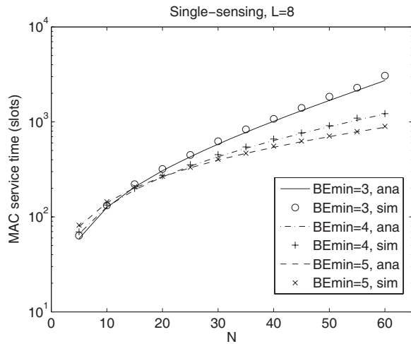
Fig. 8. Average frame service time in the SS case
