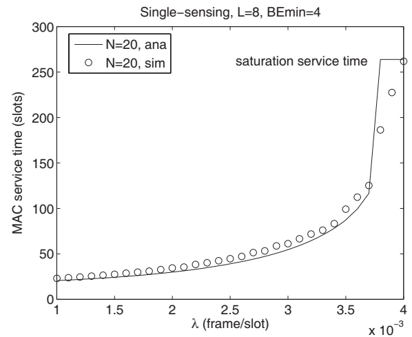
Fig. 9. Average frame service time in unsaturated case
