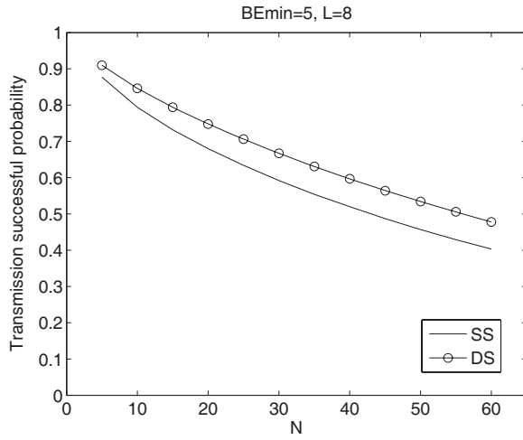
Fig. 5. Transmission successful probabilities in SS and DS cases
