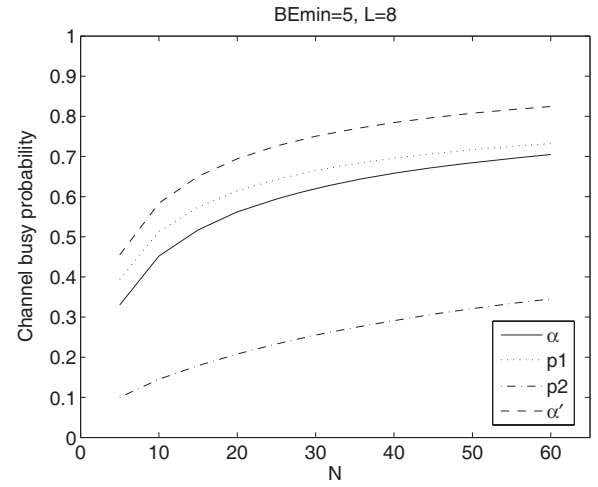
Fig. 6. Channel busy probabilities in the CCAs in SS and DS cases
