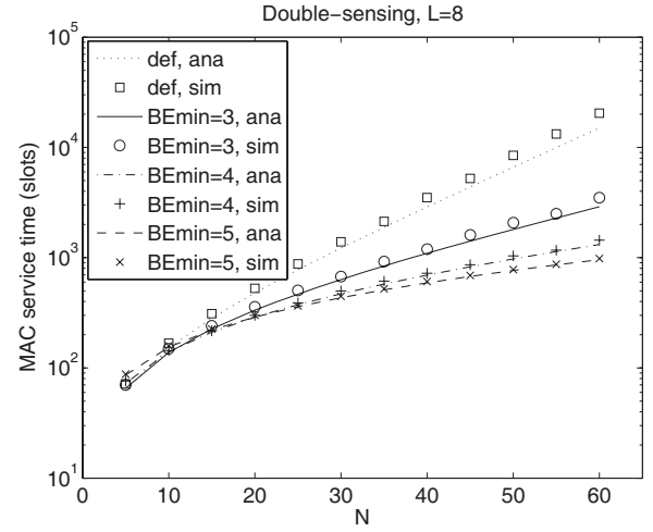
Fig. 4. Average frame service time in saturated case
