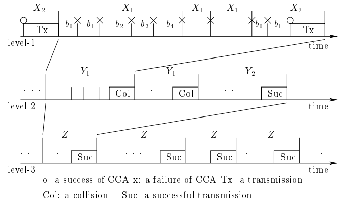
Fig. 2. Illustration of the concept of 3-level renewal process, M=5
