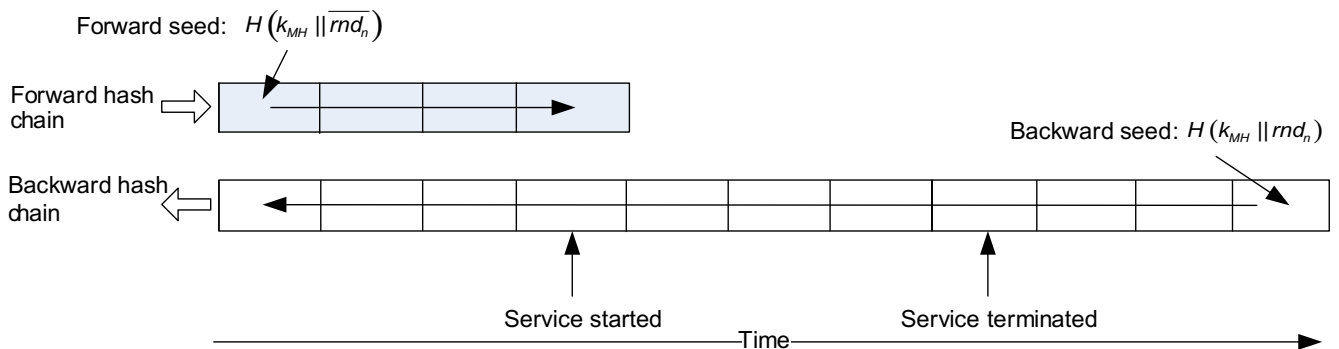
Fig. 4. MDDHC setup at MT.
