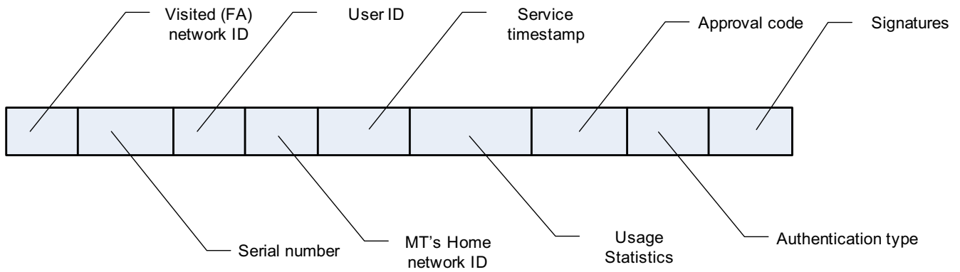
Fig. 6. Event ID data structure.
