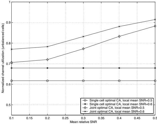
Fig. 6. Comparison of joint and single-cell channel assignments for unbalanced traffic.
