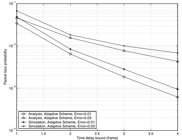
Fig. 9. Packet loss probability for the ADP scheme.
