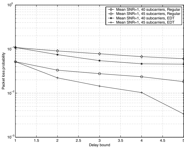
Fig. 7. Comparison of packet loss probability for the regular and EDT schemes.
