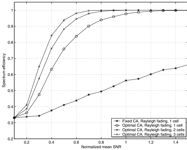
Fig. 4. Comparison of optimal assignment vs fixed assignment.
