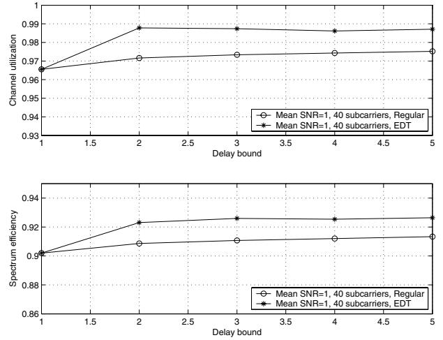
Fig. 8. Comparison of spectral efficiency/channel utilization for the regular and EDT schemes.
