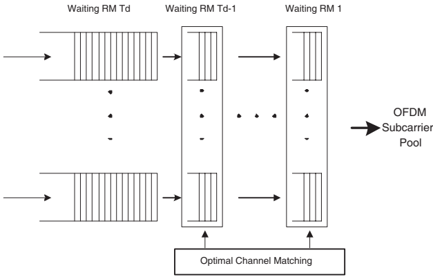
Fig. 3. Prioritized assignment based on packet delay.
