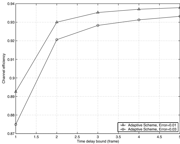
Fig. 10. Channel efficiency for the ADP scheme.
