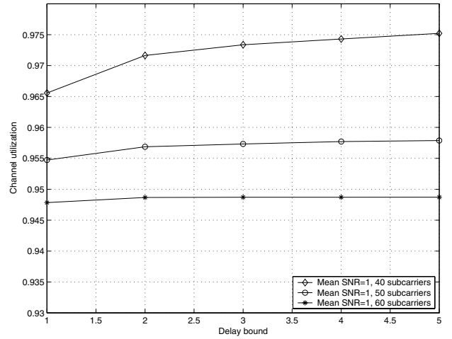
Fig. 5. Channel utilization with different number of assignable channels.
