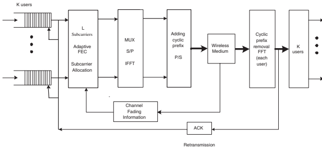
Fig. 1. Real-time video transmission over OFDM wireless channels.
