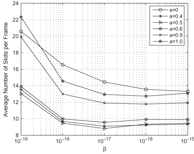
Fig. 2. Scheduling performance with respect to the different values of a ; \alpha = 0.01 .
