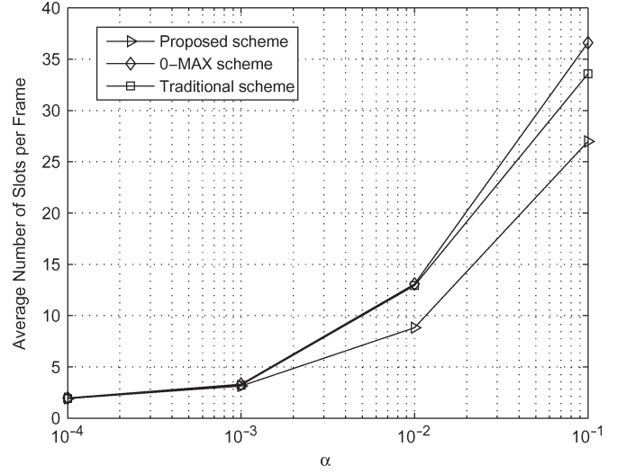
Fig. 6. Scheduling performance with respect to the different values of \alpha ; \beta = 10^{-17} .
