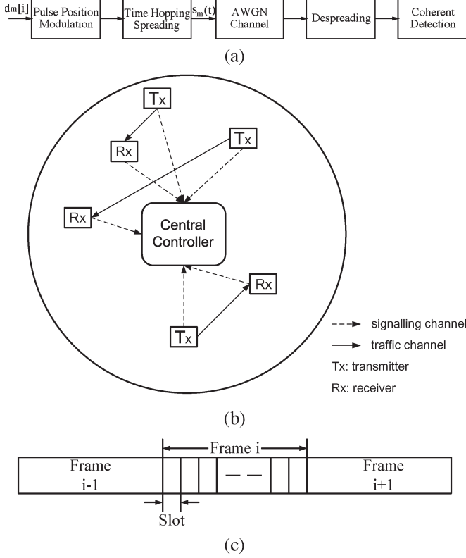
Fig. 1. System model of the UWB-based ad hoc network. (a) Physical layer model. (b) MAC layer model. (c) Frame structure.
