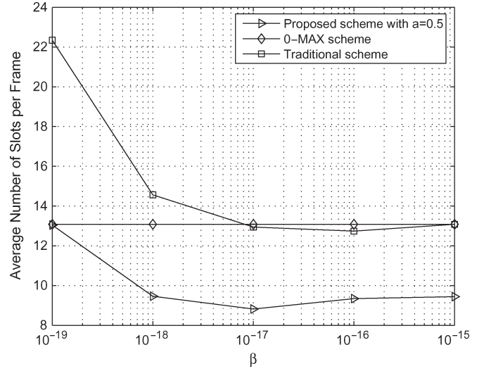
Fig. 3. Scheduling performance comparison among three scheduling schemes; \alpha = 0.01 .
