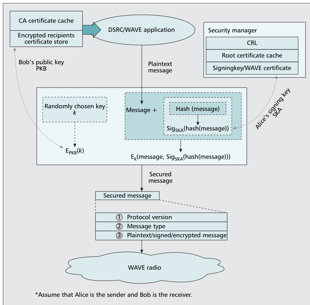
■ Figure 2. The IEEE Std 1609.2 security services framework for creating and exchanging WAVE messages between WAVE devices.
