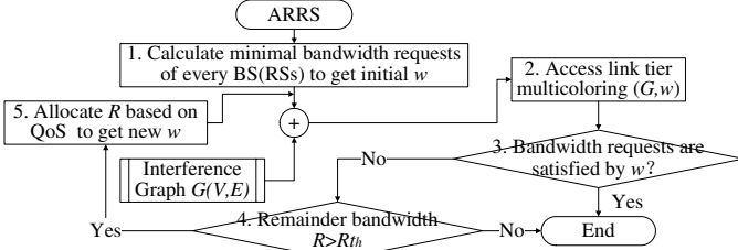
Fig. 2. Flowchart of ARRS algorithm.
