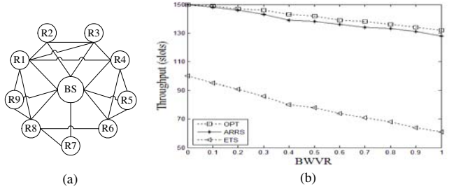
Fig. 5. Throughput vs. BWVR of nine RSs scenario.
