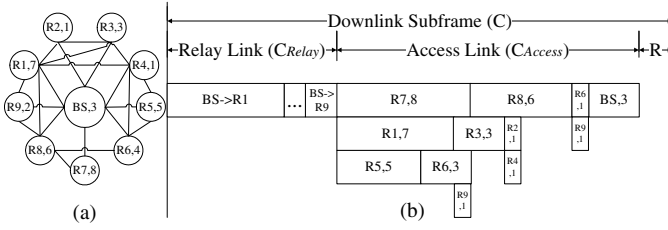
Fig. 1. Example of scheduling model and scheduling result.
