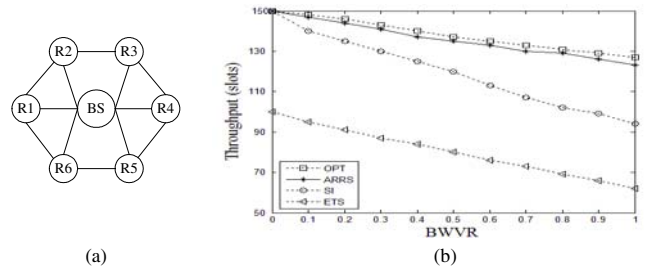
Fig. 4. Throughput vs. BWVR of six RSs scenario.
