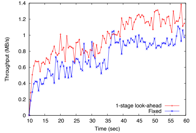
Fig. 16. A random topology with 15 secondary flows ( p = 0.4 in 10s-35s, p = 0.8 in 35s-60s).
