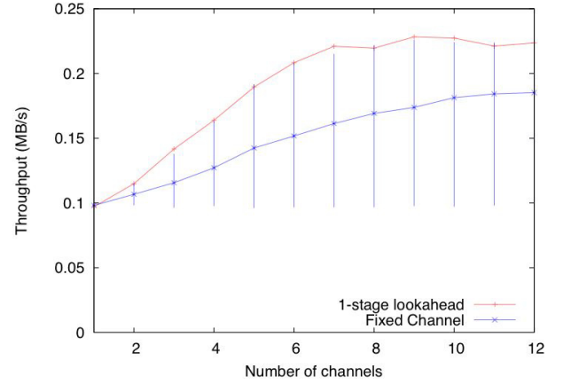
Fig. 9. The throughput with different total numbers of channels.
