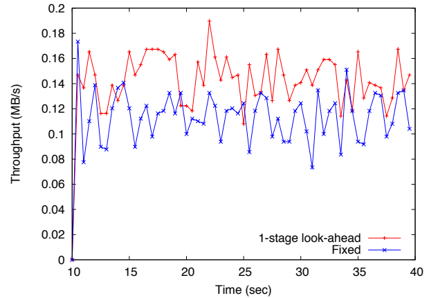
(b) Throughput of flow 3-4.
