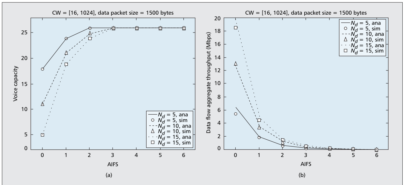
■ Figure 2. Parameters of VoIP over WLAN.
