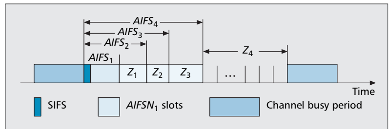
Figure 1. An illustration of prioritized channel access for different station classes.
