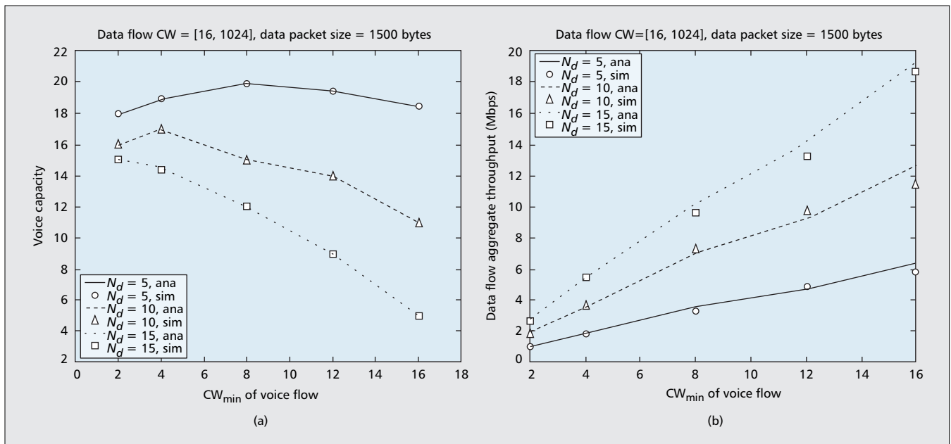
Figure 3. Effect of AIFS in ad hoc mode.
