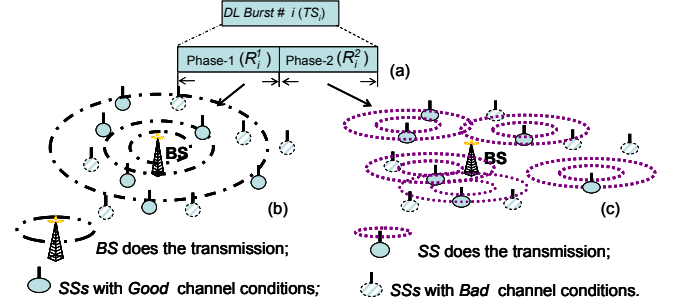
Fig. 3. The illustration of the cooperative multicast scheduling.
