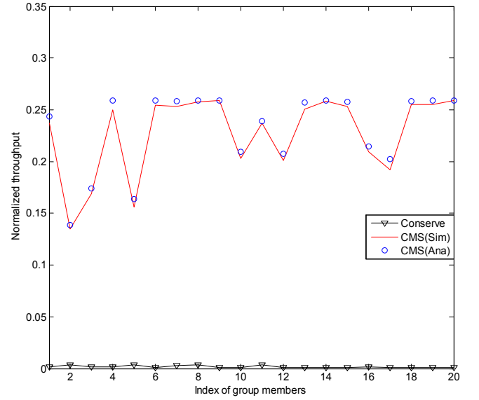
Fig. 5. Throughput of each group member with AMC.
