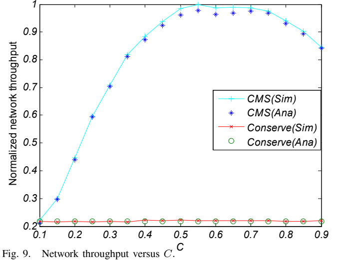
Fig. 9. Network throughput versus C .
