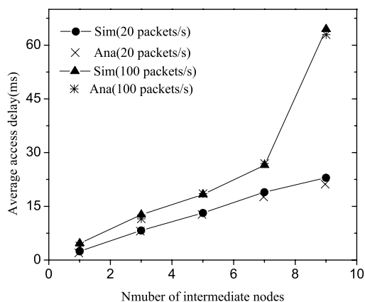
Fig. 9. Access delay for RMNs.
