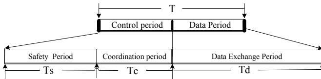
Fig. 4. Timing structure.
