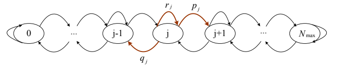
Fig. 6. State transition of a ring modeled by Markov chain.
