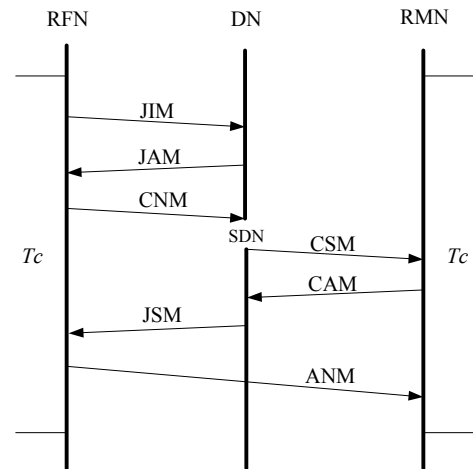
Fig. 5. Illustration of the joining process.
