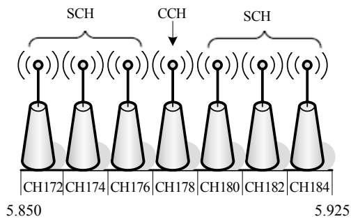
Fig. 1. Multi-channel structure.
