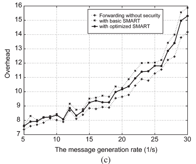
Fig. 6. Impact of network load on system performance. (a) Successful delivery ratio. (b) Average latency. (c) Overhead ratio.
