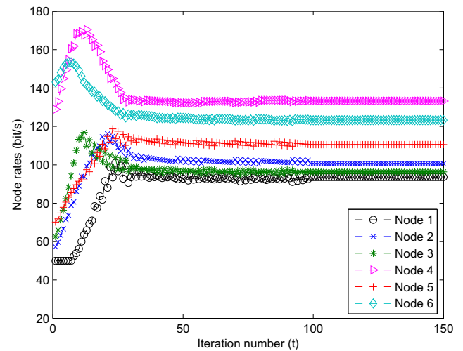
Fig. 4. The convergent performance of the Algorithm DAULT , \gamma = 0.95 .
