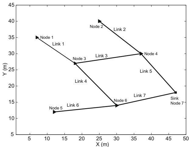
Fig. 2. Topology of a wireless sensor network.
