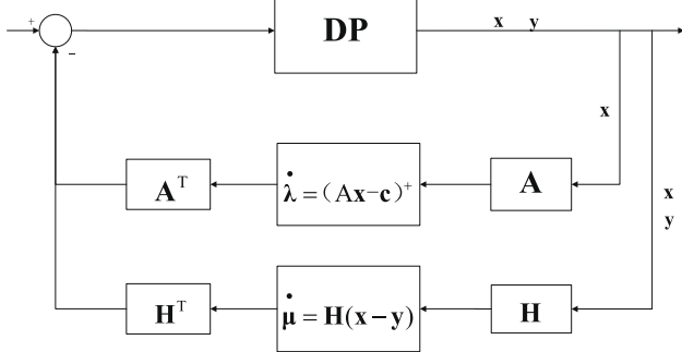
Fig. 1. Close-loop system framework of algorithm DAULT.
