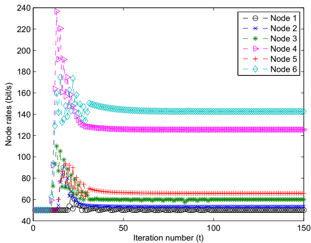
Fig. 5. The convergent performance of the Algorithm DAULT, \gamma = 0.1 .
