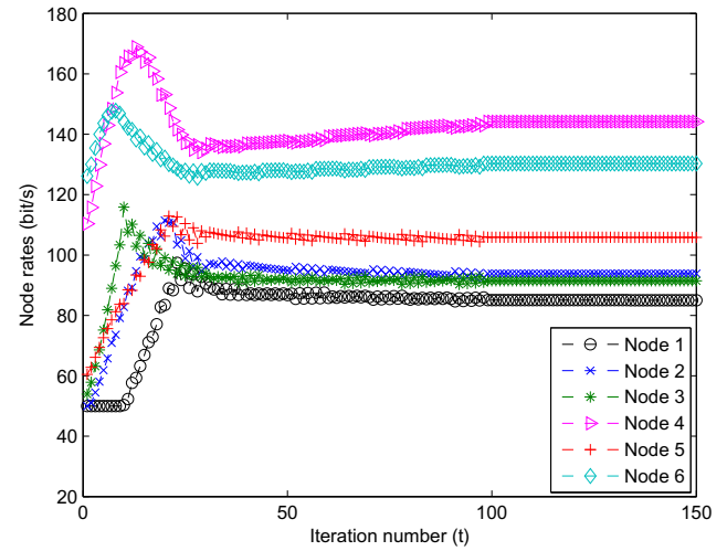
Fig. 3. The convergent performance of the Algorithm DAULT , \gamma = 0.8 .
