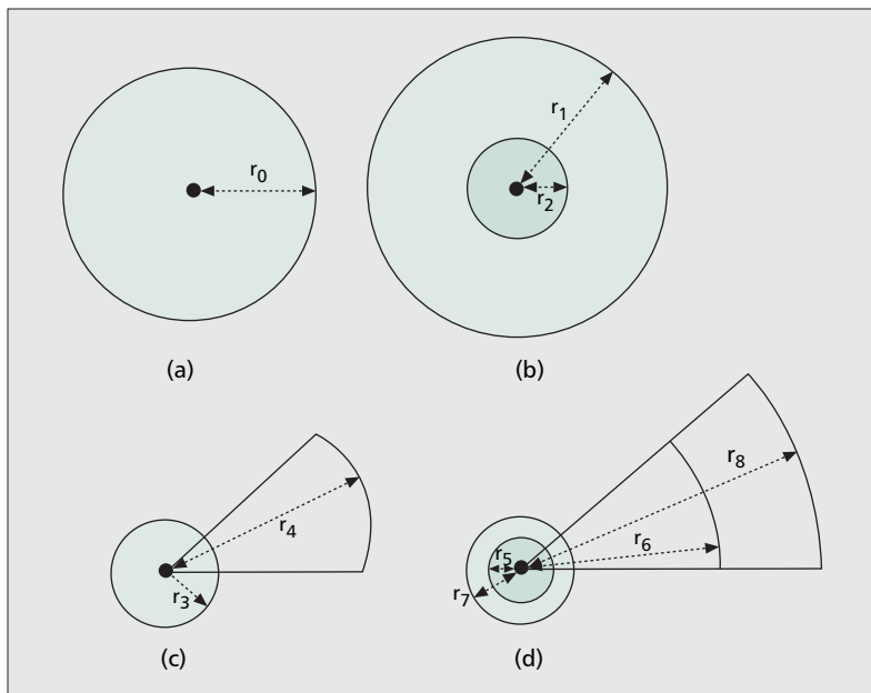
■ Figure 3. Exclusive Regions: a) omni-omni; b) directional-omni; c) omni-directional; d) directional-directional.
