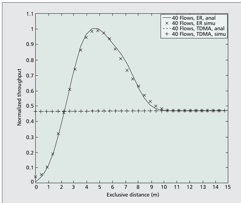
■ Figure 5. Network throughput under various ER sizes.
