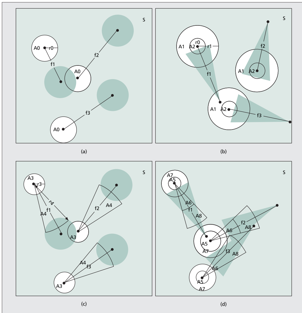
■ Figure 4. Concurrent transmissions: a) omni-omni; b) directional-omni; c) omni-directional; d) directional-directional.
