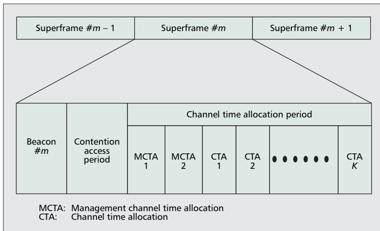
■ Figure 1. IEEE 802.15.3 superframe structure.
