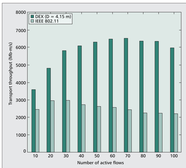
■ Figure 6. Network transport throughput comparison.
