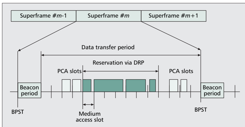
■ Figure 2. WiMedia MAC superframe structure.
