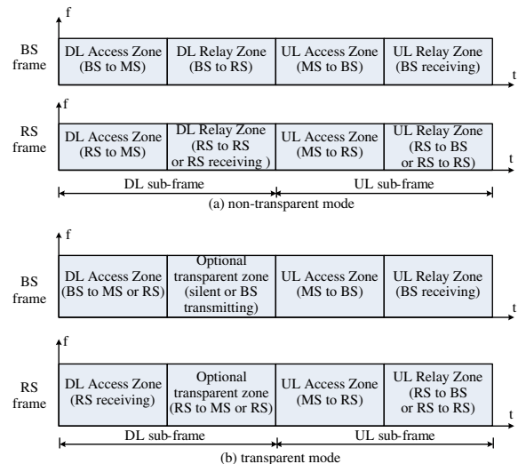
Fig. 2. IEEE 802.16j frame structure.
