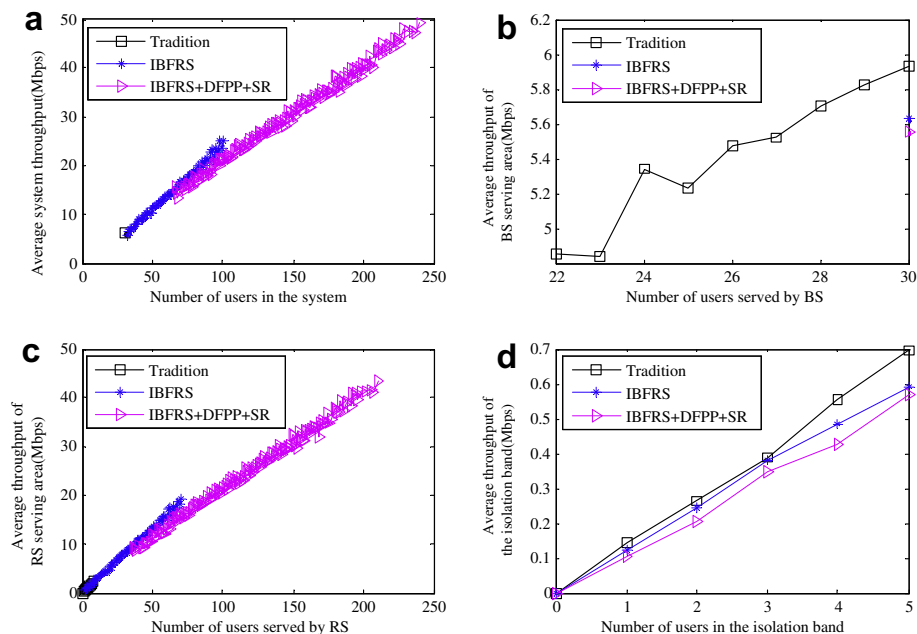
Fig. 8. Throughput comparison.
