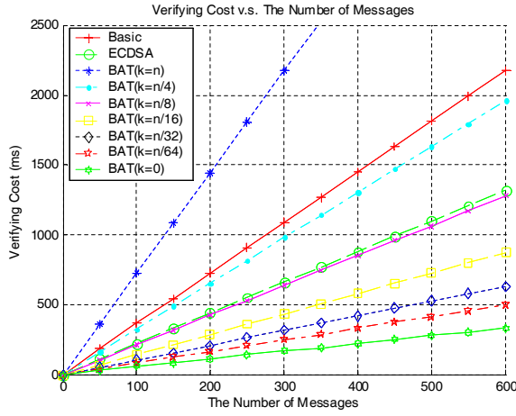
Fig. 3. Verification cost vs. number of messages ( n : the number of messages, k : the number of bogus messages).
