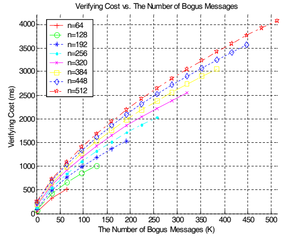
Fig. 4. Verification cost of BAT scheme vs. number of bogus messages ( k : the number of bogus messages).
