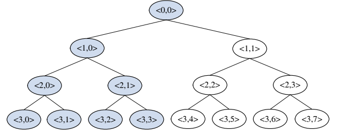
Fig. 5. BAT with bogus signatures.
