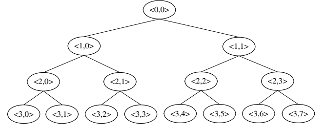
Fig. 2. Binary authentication tree.
