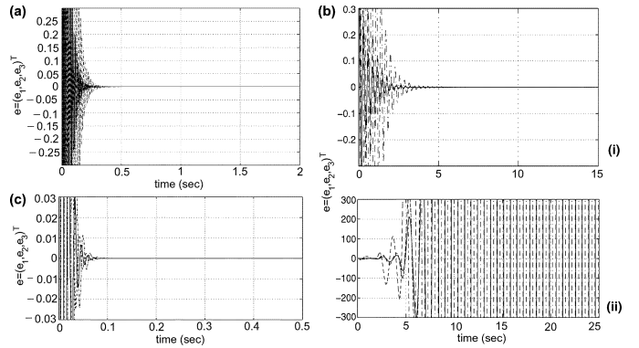
Fig. 4. (a) IS of two Chua's oscillators with \mathbf{B} = -0.7\mathbf{I} and r = 0.003 . (b) IS of two Chua's oscillators: (i) \mathbf{B} = -0.03\mathbf{I} and r = 0.07 ; (ii) \mathbf{B} = -0.002\mathbf{I} and r = 2 . (c) IS of two Chua's oscillators with \mathbf{B} = -\mathbf{I} , r = 0.003 and \Delta = 0.001 .
