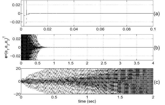
Fig. 3. IS of two Chua's oscillators with different delay values (a) r = 0.0011 . (b) r = 0.0021 . (c) r = 0.003 .
